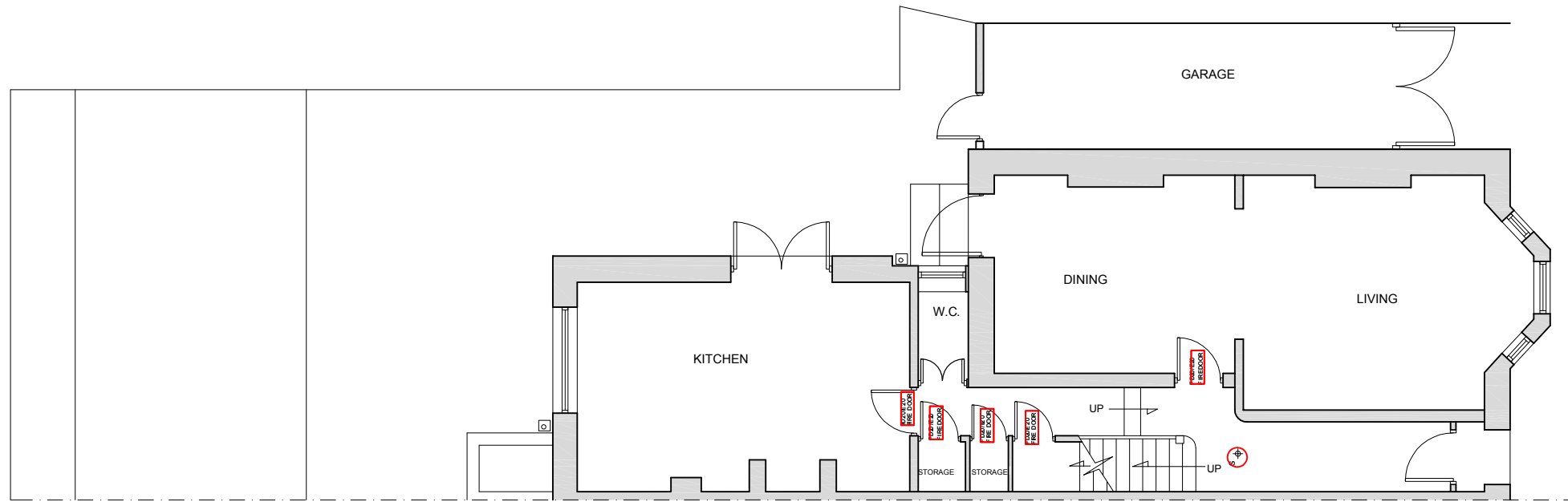
Proposed Ground Floor Plan (Unchanged)
