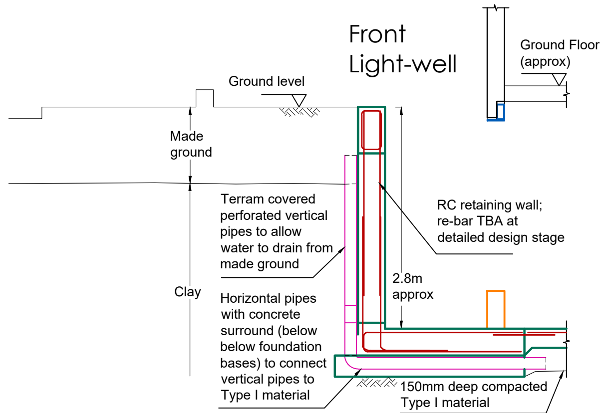
Section 1-1
