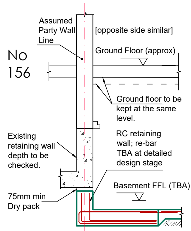
Section 2-2
