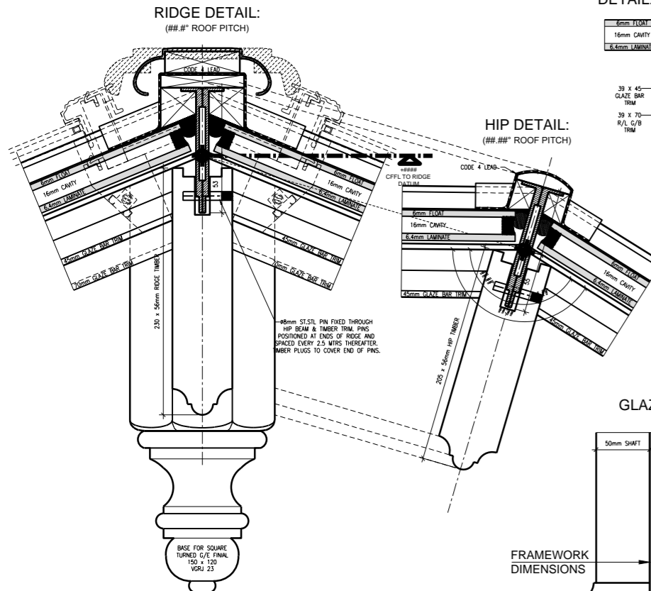
RIDGE DETAIL: (88.8° ROOF PITCH)
