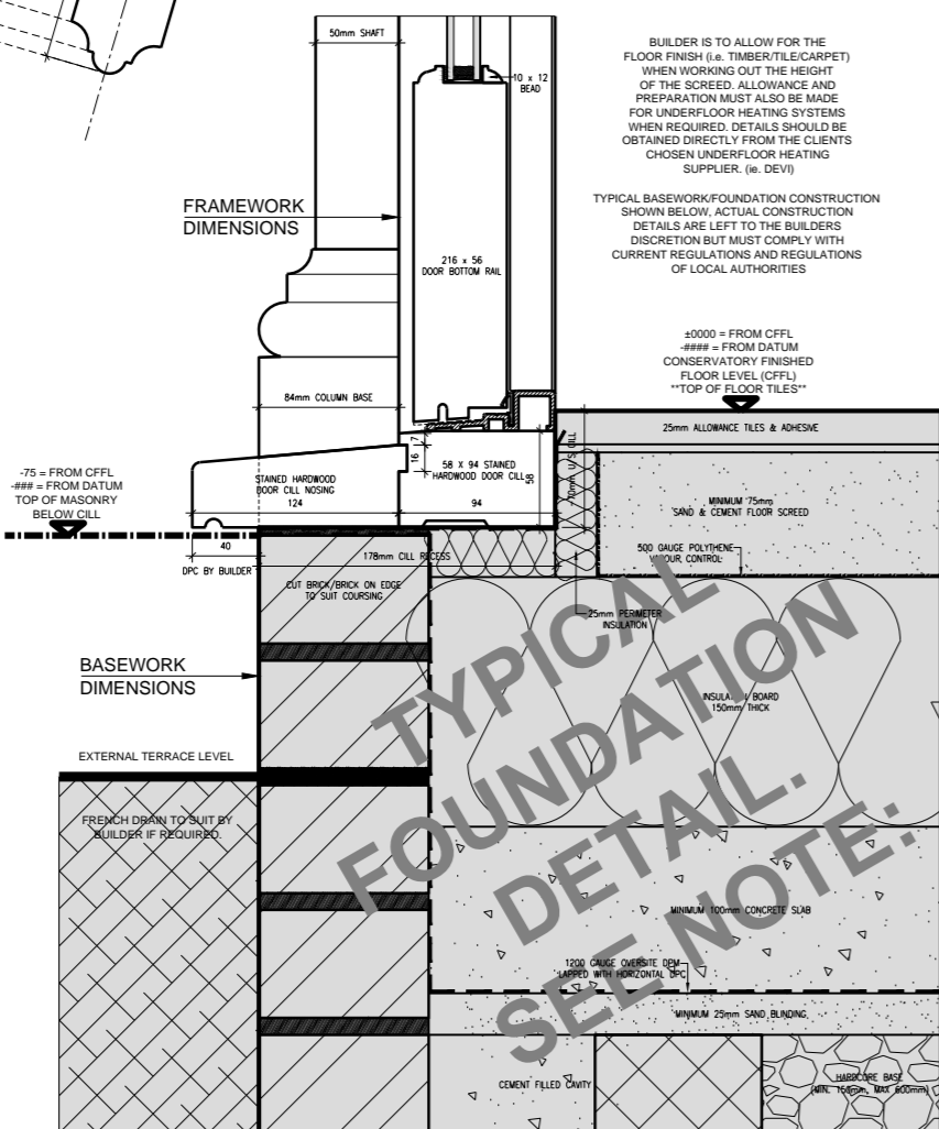
FULL HEIGHT GLAZED DOOR PANEL
