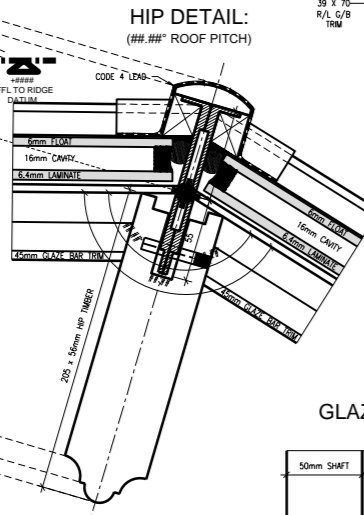
HIP DETAIL: (88.8° ROOF PITCH)
