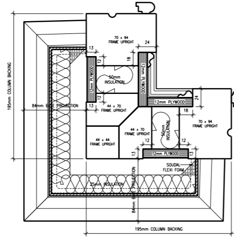
FULL HEIGHT GLAZED FIXED PANEL
