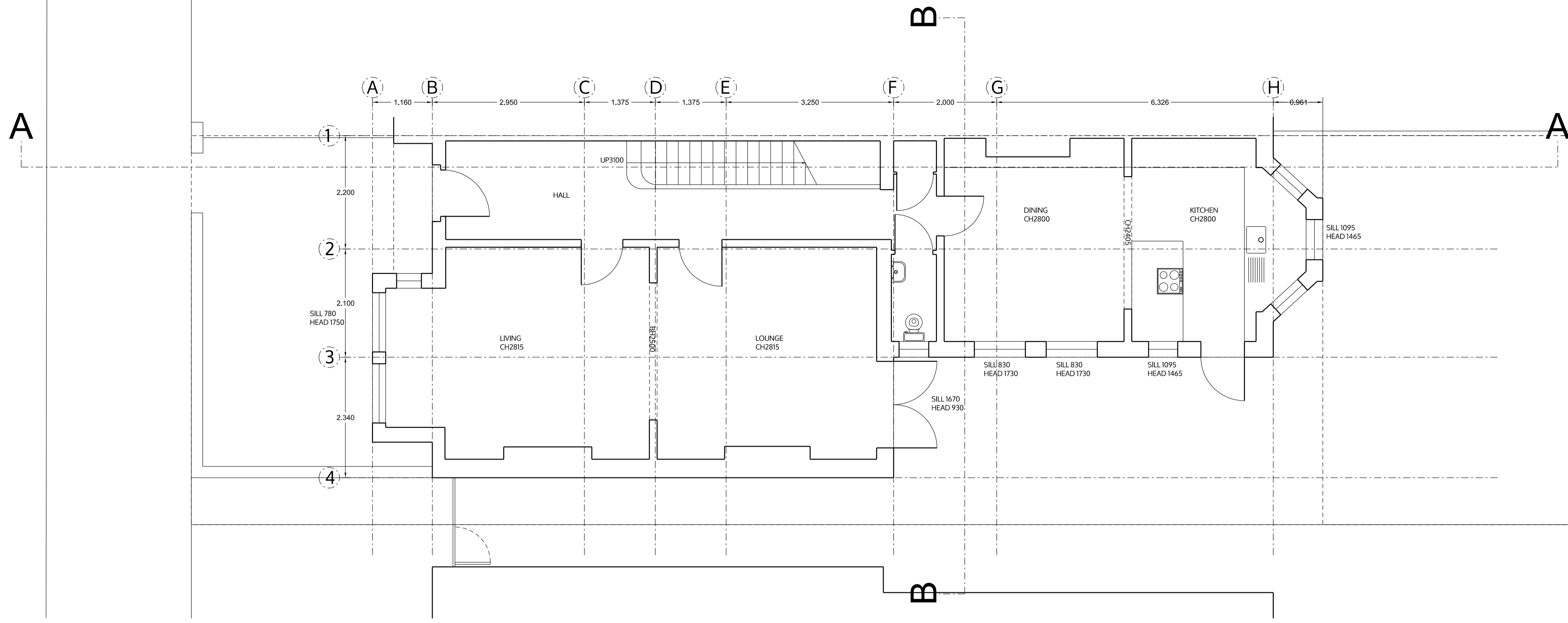
GROUND FLOOR
