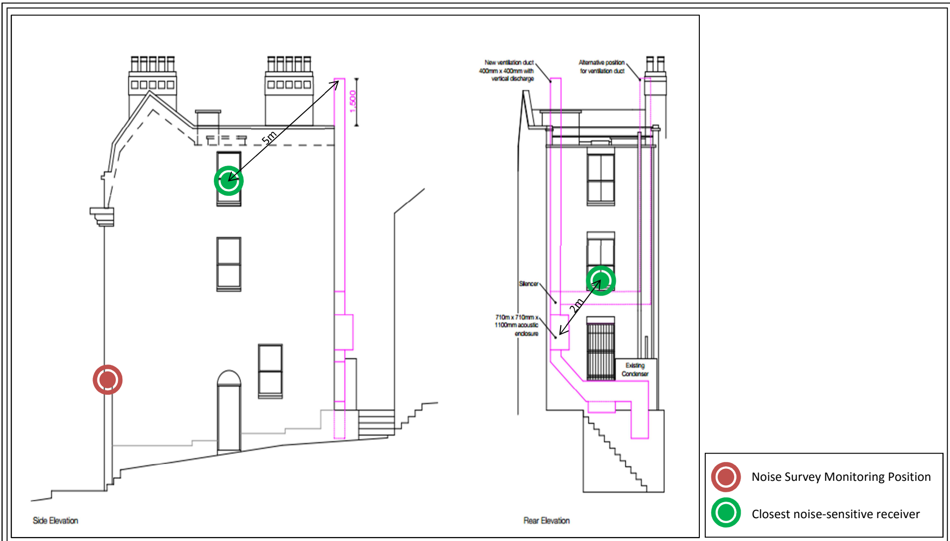
Title: Indicative site plan showing noise monitoring position (Image Source: Emily Greeves Architects)
