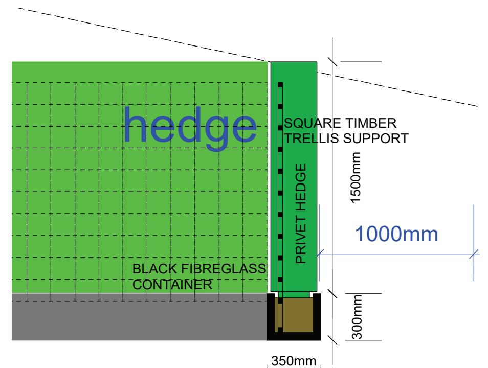
SECTION THROUGH HEDGE & CONTAINER SCREEN : 1:25 scale
