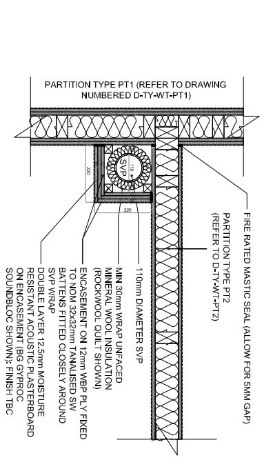
D-J-WT-704.2 - PLAN DETAIL - SVP BOXING PT1/PT2
