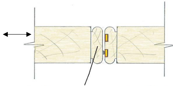
New european oak edges with staff bead profile and now incorporating intumescent seals 1 x fire only and 1 x fire / smoke.
