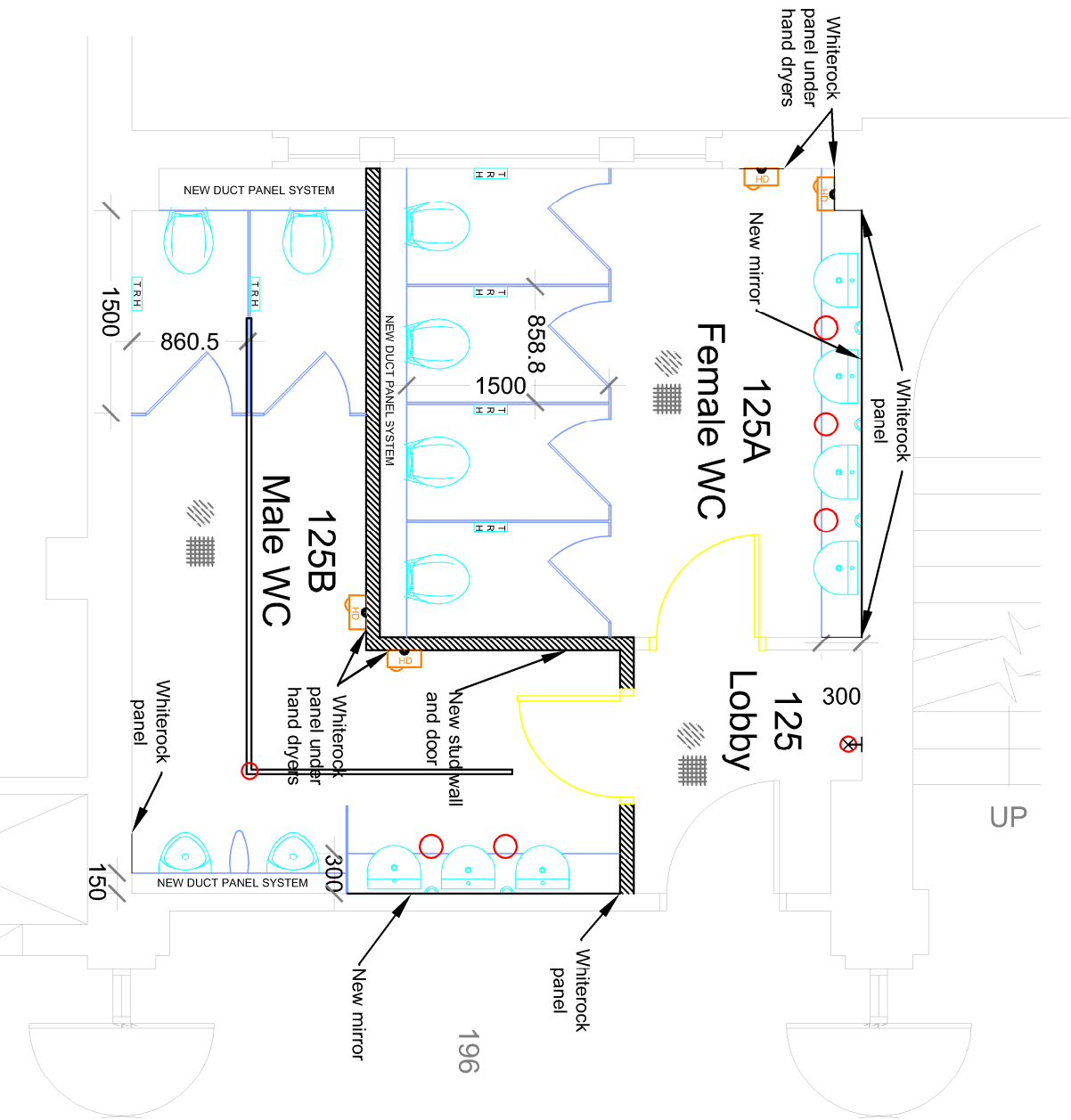
3 Proposed Plan - Female WC 125A & Male WC 125B 1 : 50 @ A3
