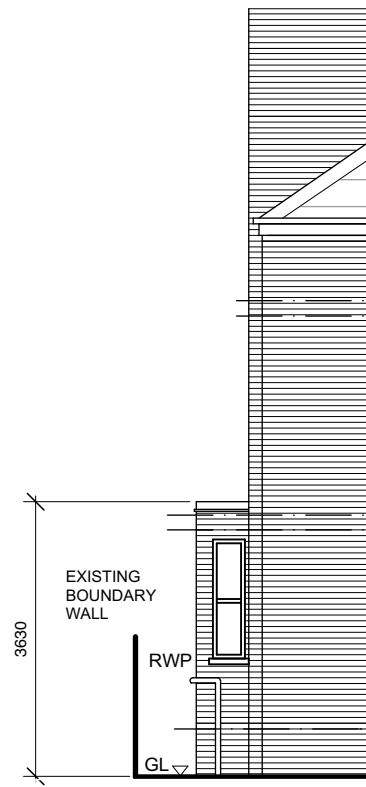
EXISTING PARTIAL SOUTH ELEVATION
