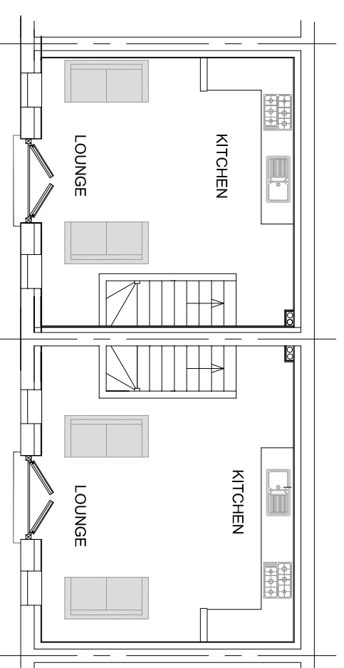
FIRST FLOOR PLAN No 16
