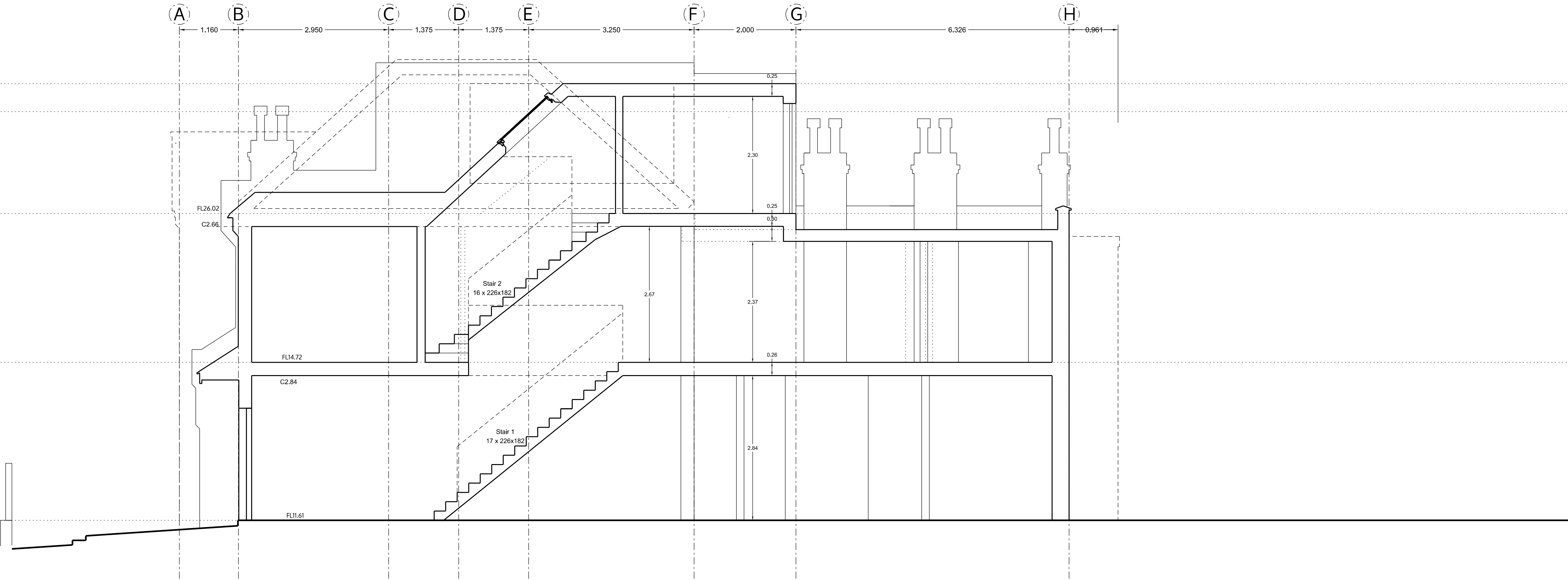
SECTION AA
