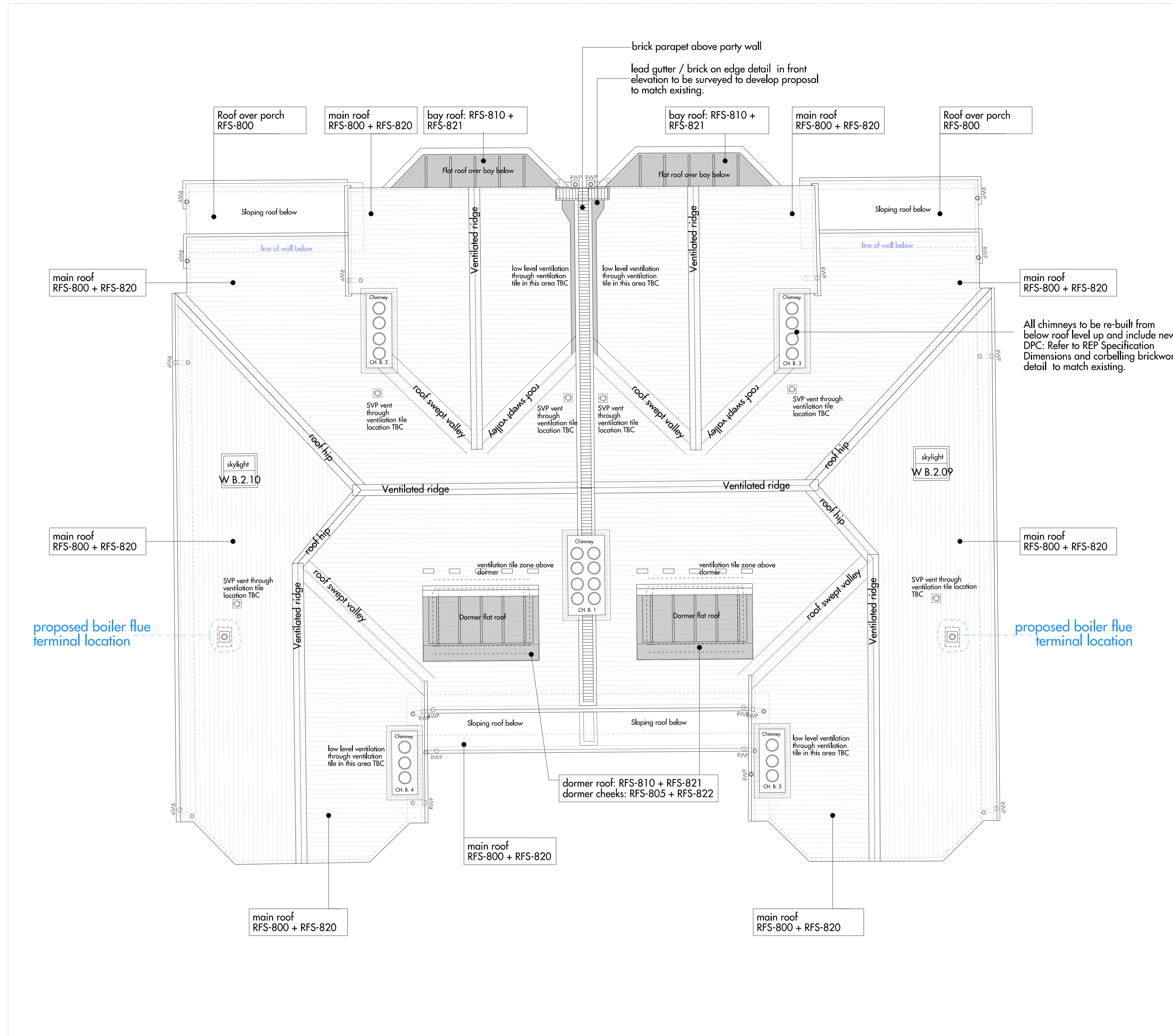
01 BLOCK B / ROOF PLAN
