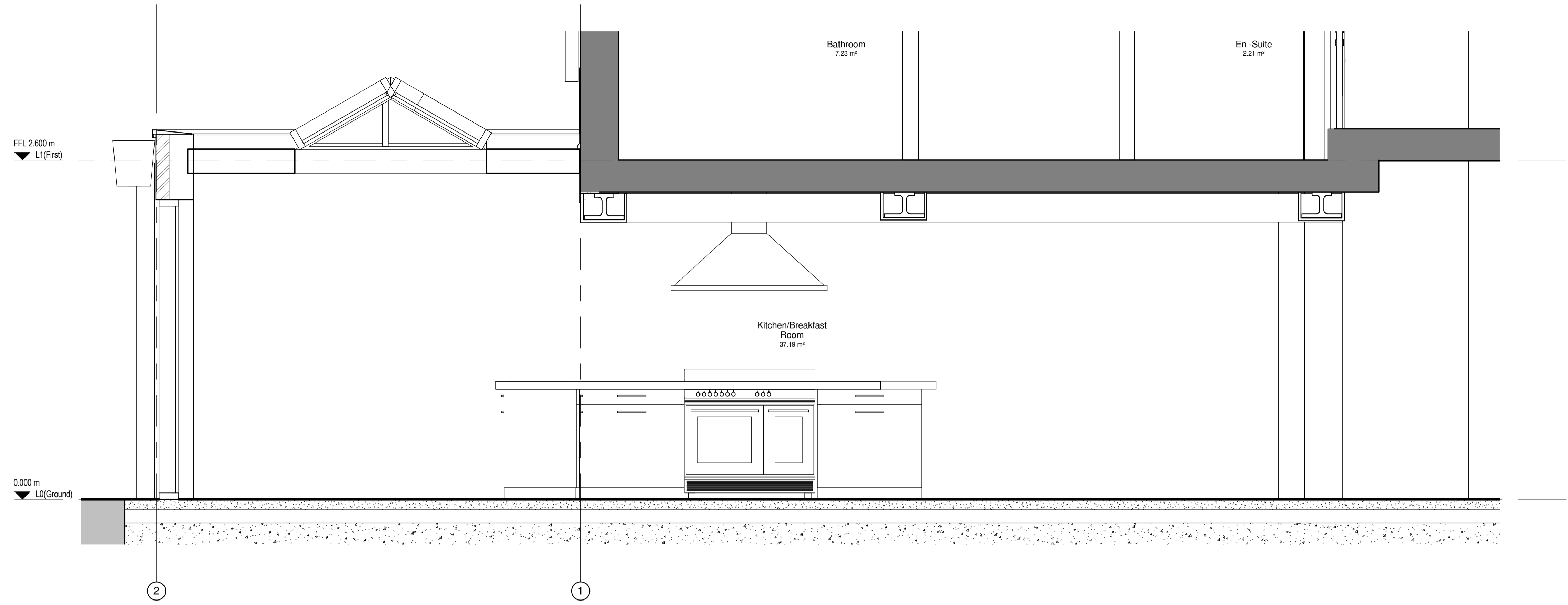
3.4 Elevation 3.4 1:20
