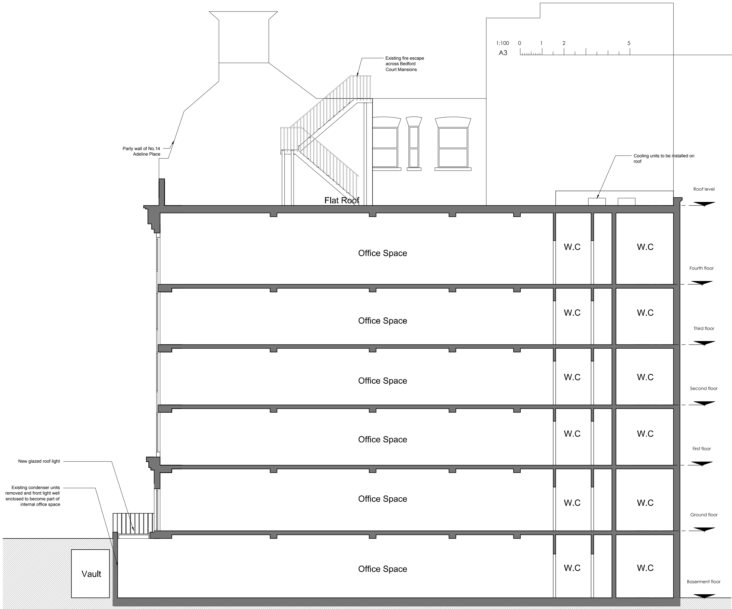
1 Section AA, proposed
