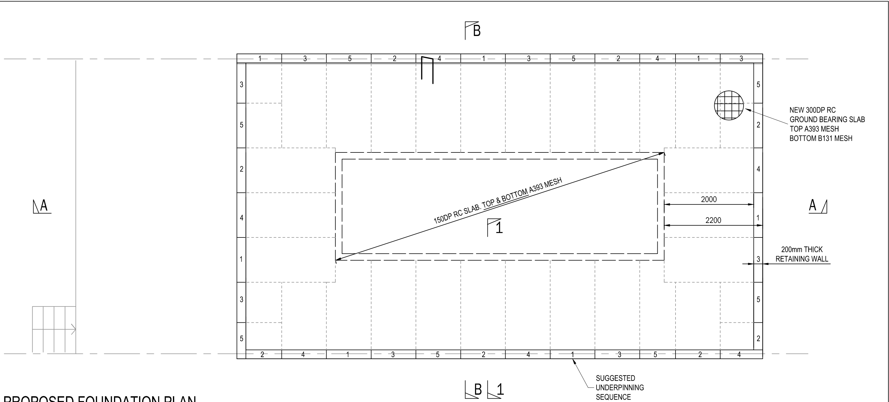
PROPOSED FOUNDATION PLAN SCALE 1:50
