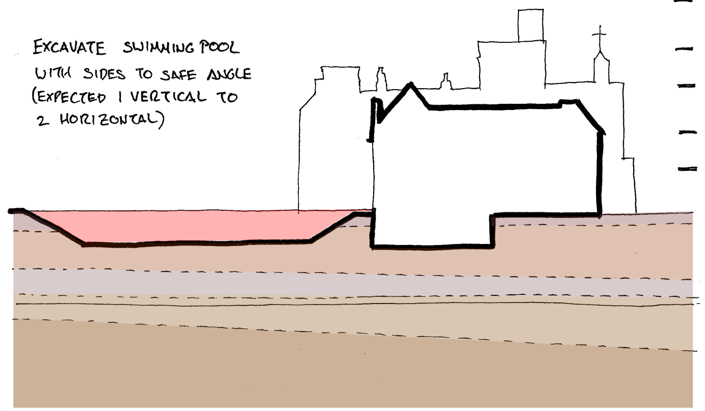
DD BASEMENT CONSTRUCTION STAGE 2
