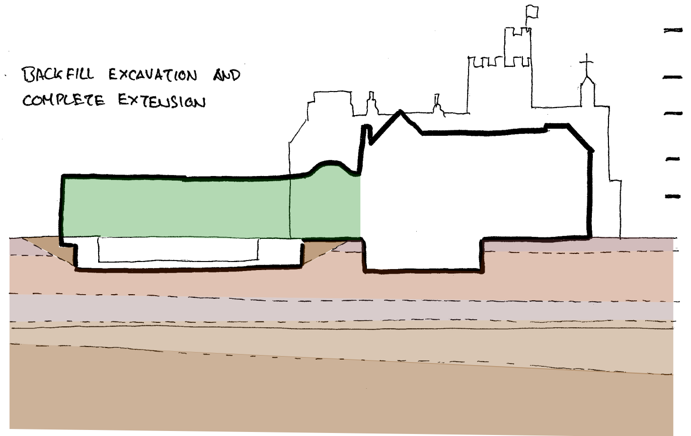
DD BASEMENT CONSTRUCTION STAGE 4
