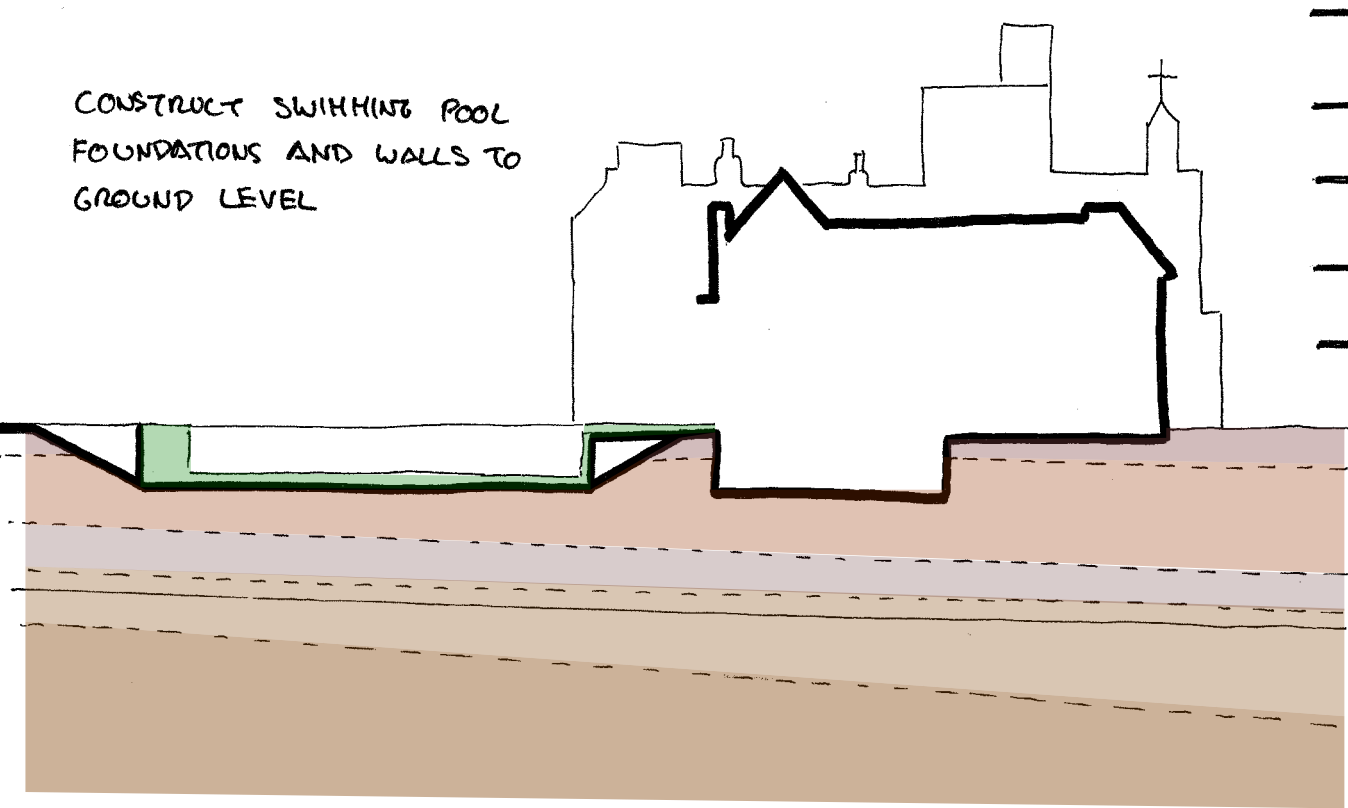
DD BASEMENT CONSTRUCTION STAGE 3
