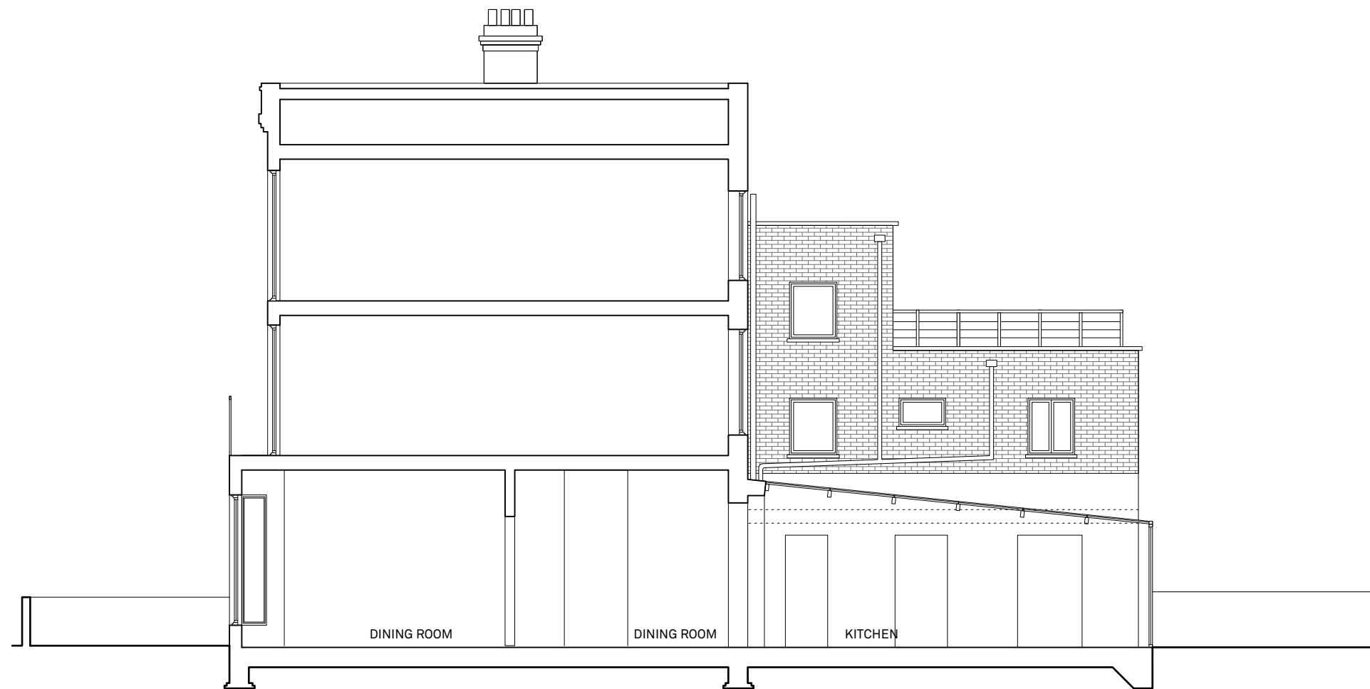
PROPOSED SECTION AA scale 1/100
