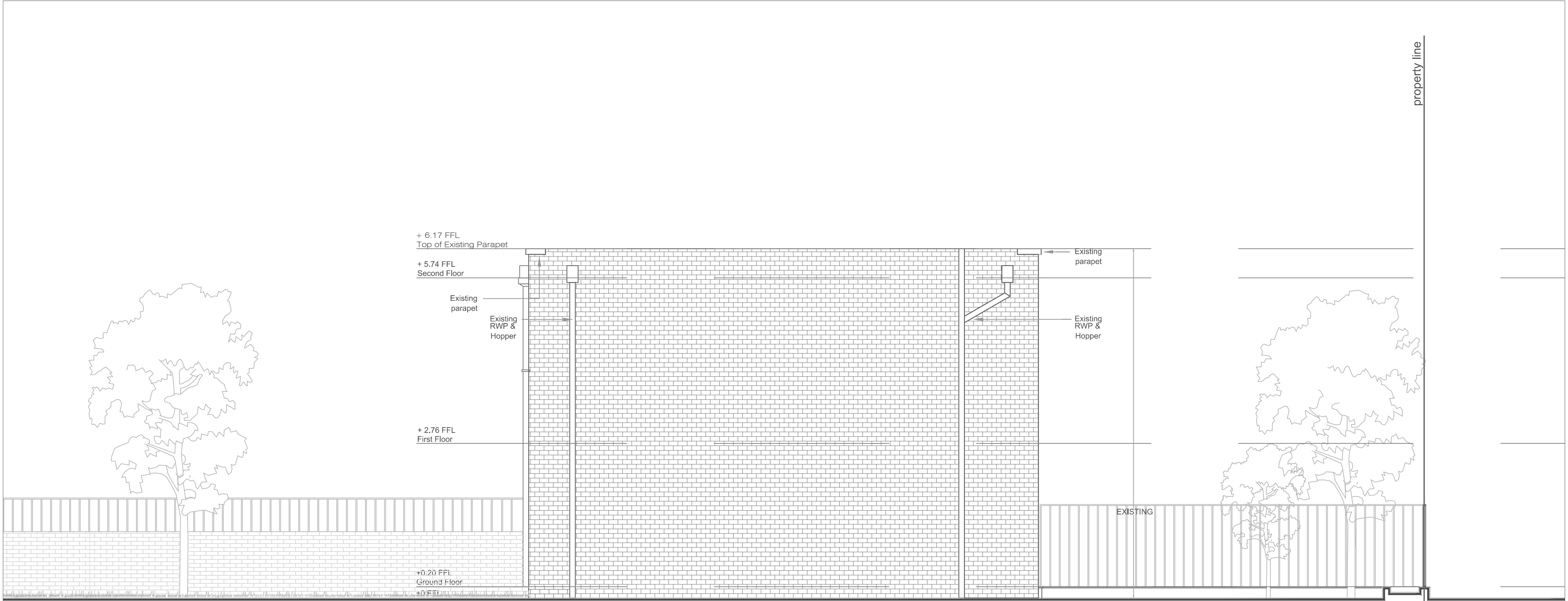
05 EXISTING SIDE ELEVATION TO 32-34 1:50
