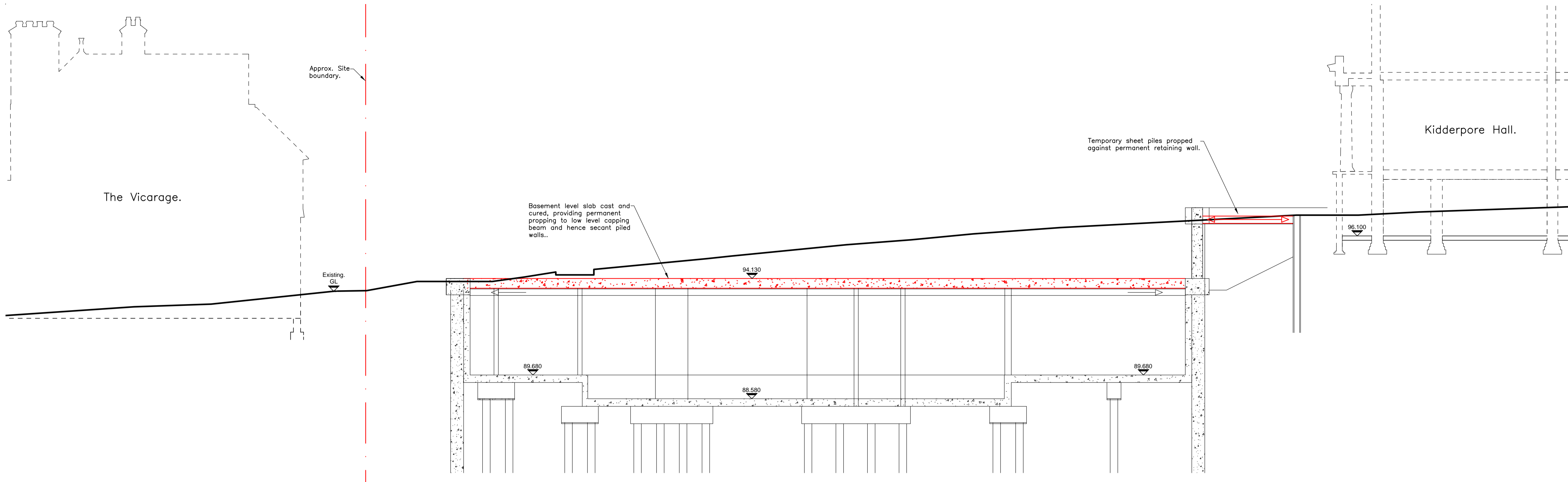
Section A-A: Construction Stage 4.
