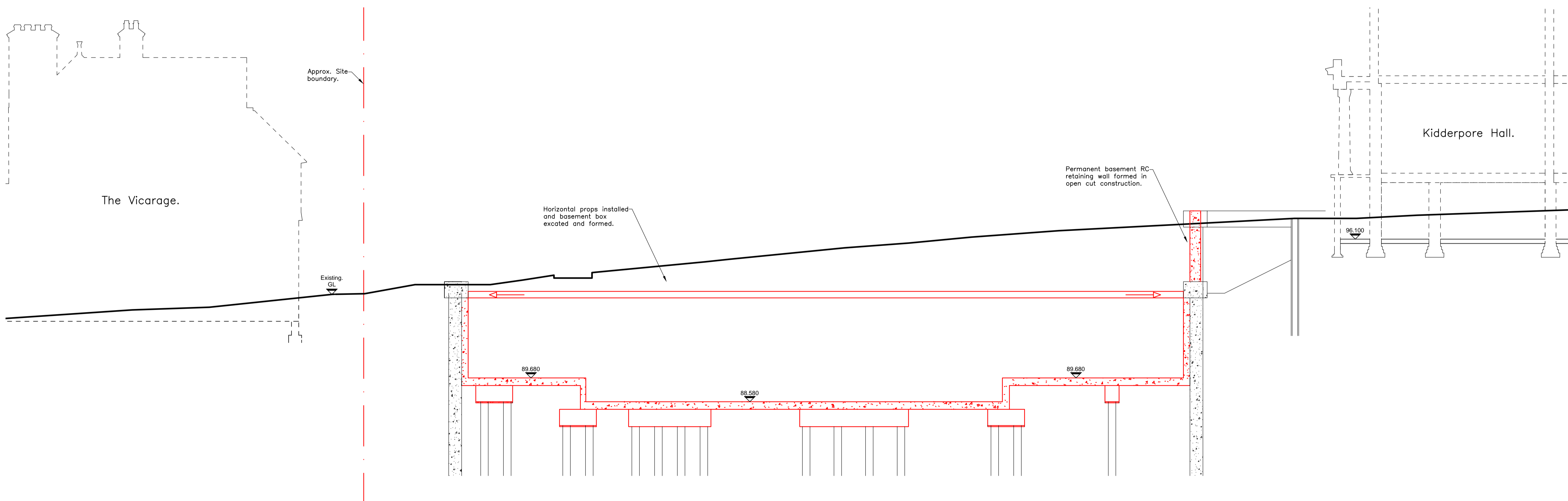
Section A-A: Construction Stage 3.
