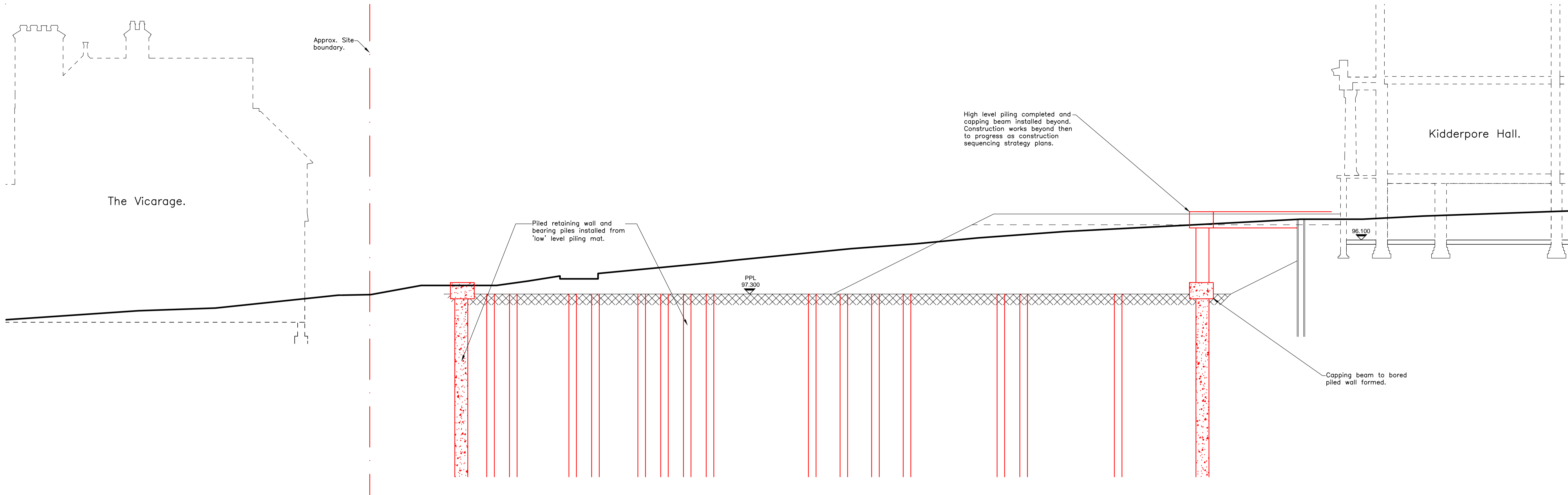
Section A-A: Construction Stage 2.
