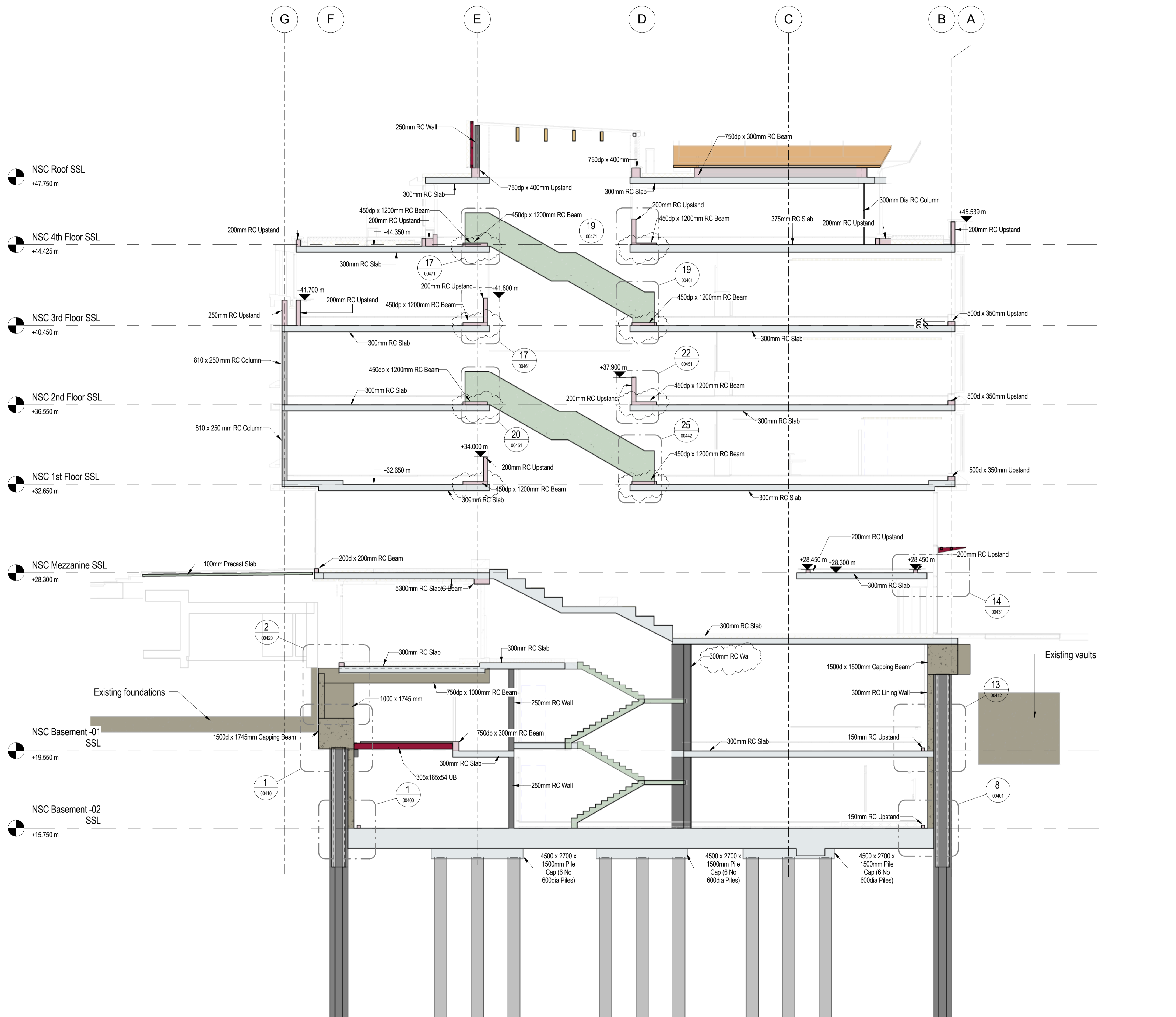
SECTION AA 1:100
