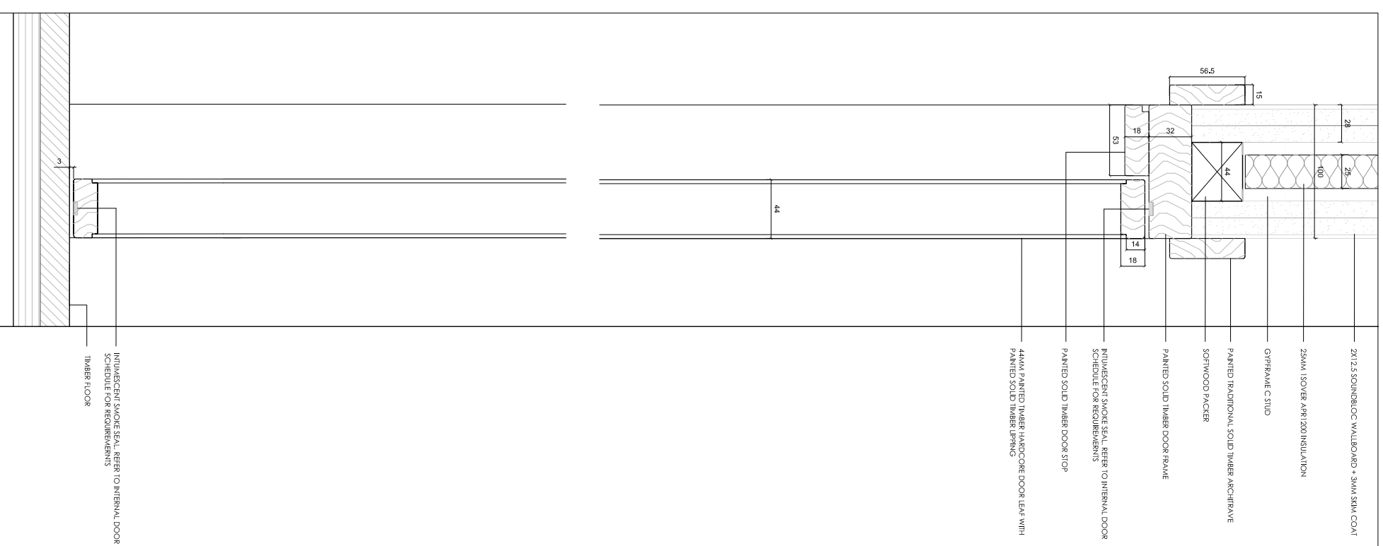
2 Flush Internal Door - Typical Head and Cill Detail SCALE 1:20@A1
