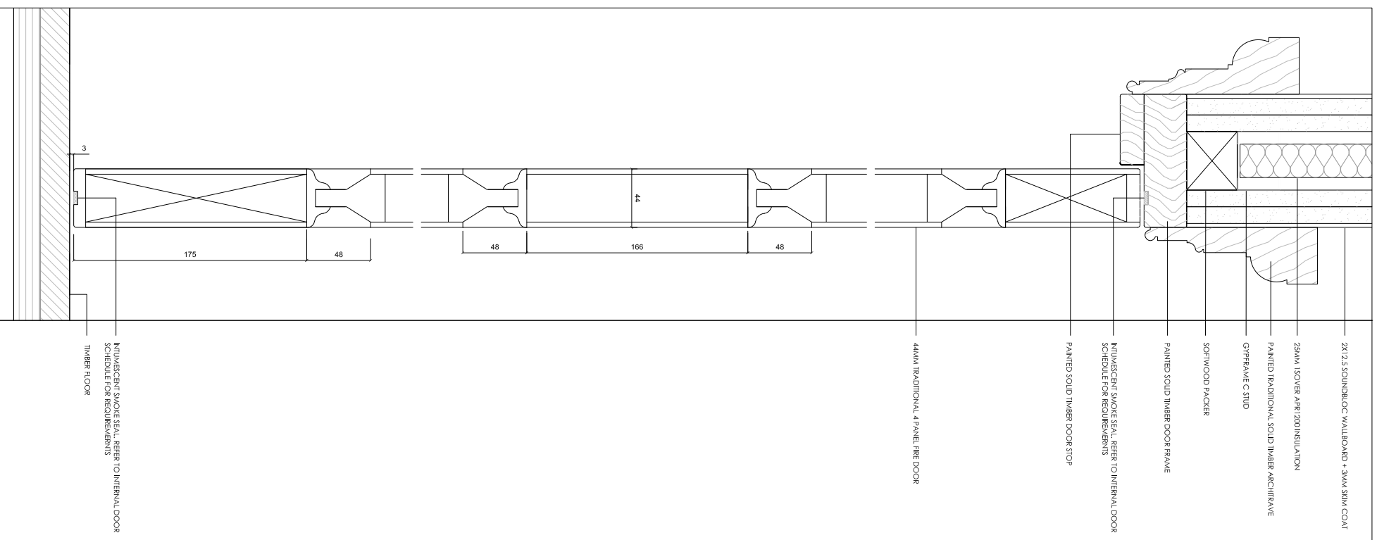
1 Traditional 4 Panel Internal Door FD30 - Typical Head and Cill Detail SCALE 1:20@A1
