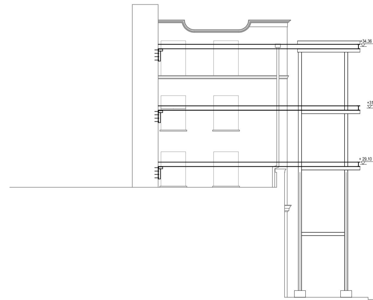
SIDE ELEVATION
