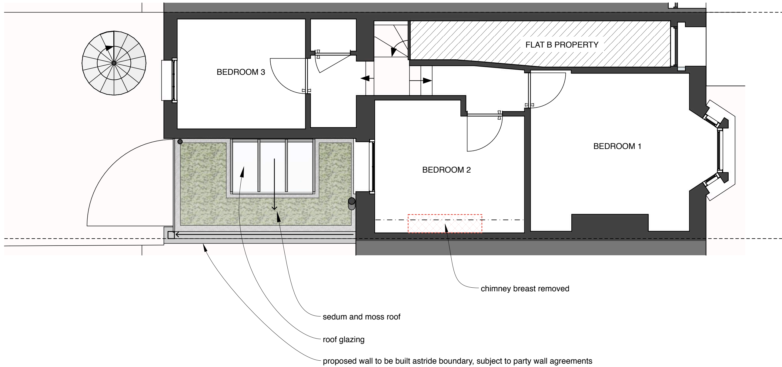
A Proposed Upper Ground Floor Plan DD07 1:50
