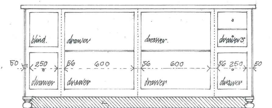
WEST FACE
