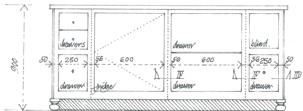
EAST FACE
