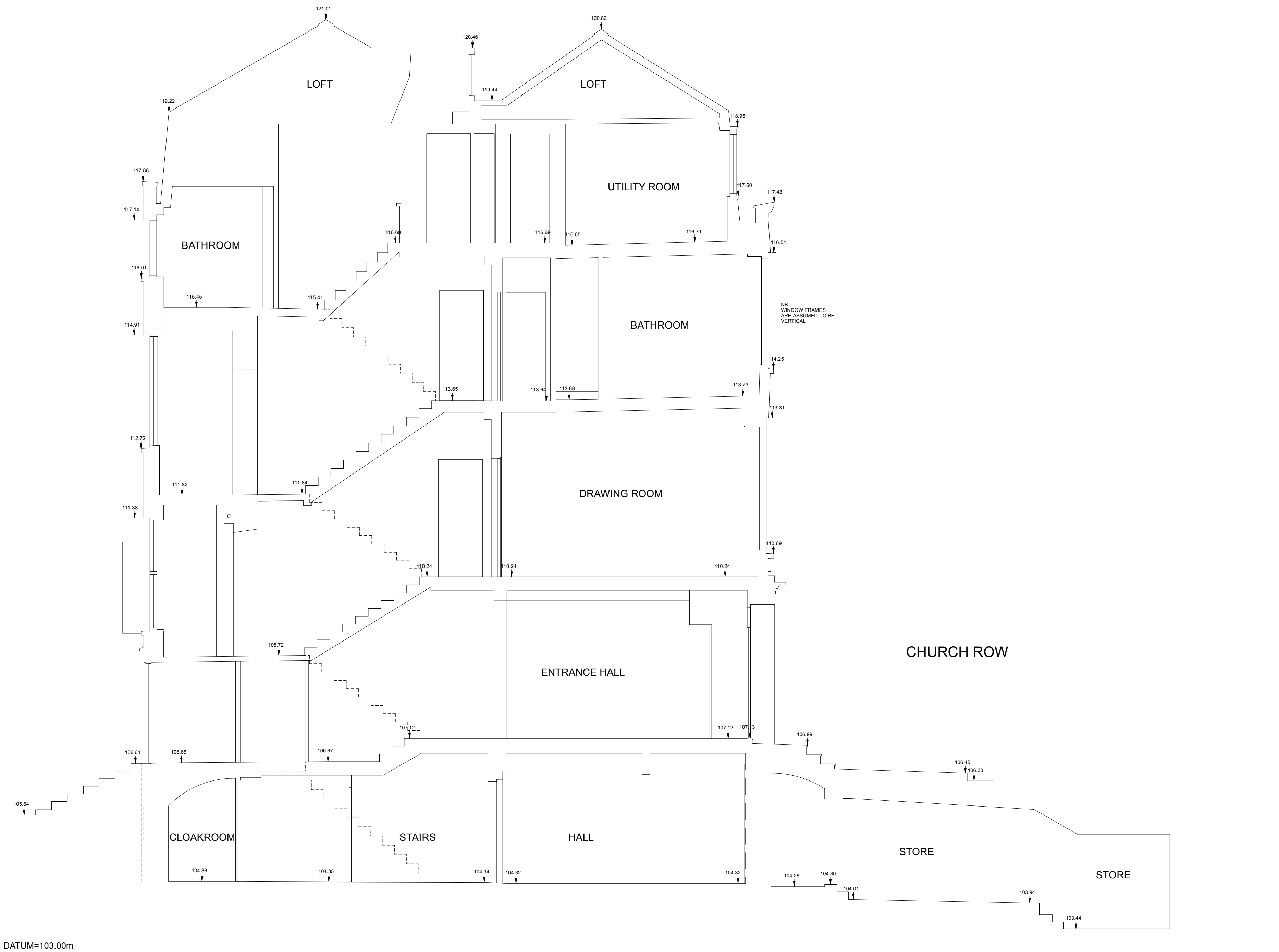
SECTION AA
