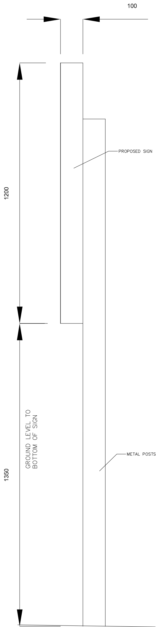
② SECTION OF PROPOSED SIGN 1:10 @ A3
