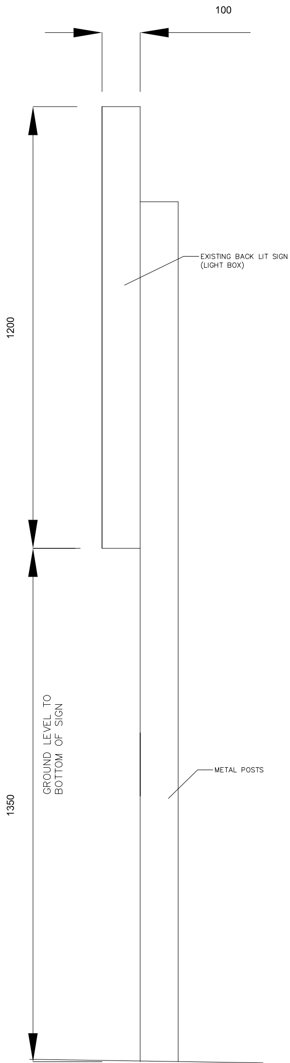
① SECTION OF EXISTING SIGN 1:10 @ A3
