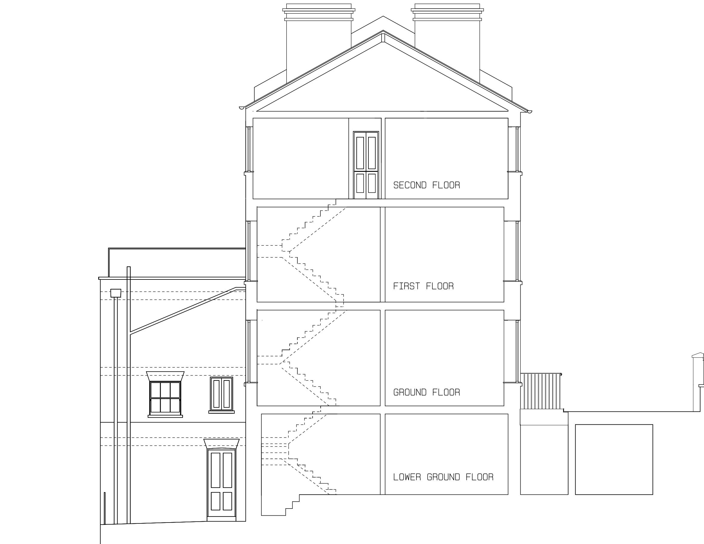
SECTION A - A ( TO NO 88 )
