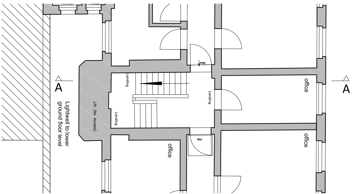
01 Lower Ground Floor E1000 SCALE 1:150
