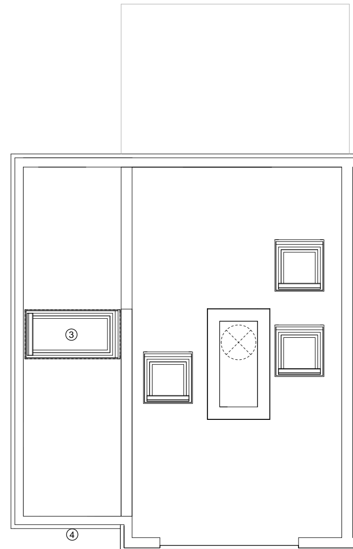
ROOF PLAN 1:100
