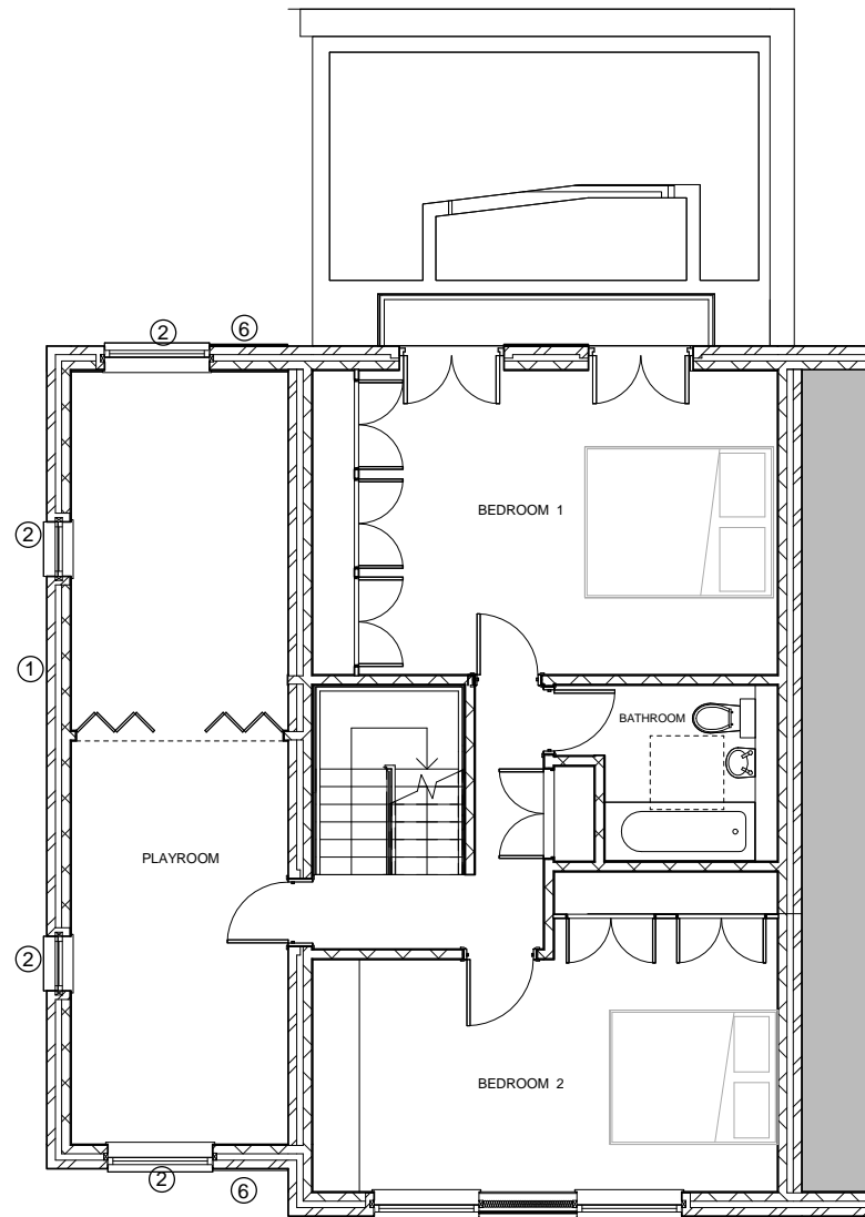
1ST FLOOR PLAN 1:100
