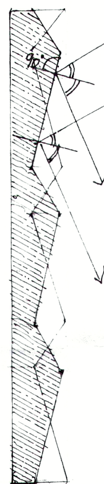
TYPICAL SECTION 1:10 OF PORTLAND STONE FACETED PANEL
