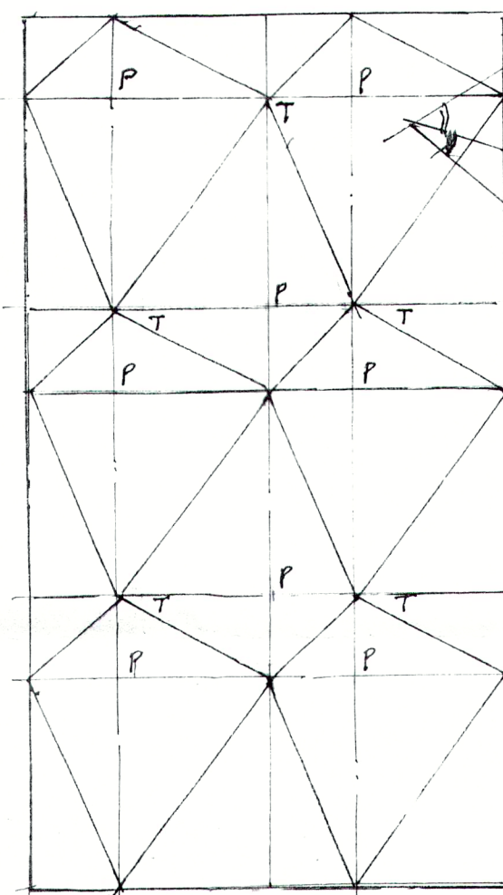
TYPICAL PART ELEVATION 1:10 OF PORTLAND STONE FACETED PANEL
