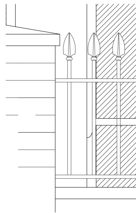
1:10 Detail of Railings
