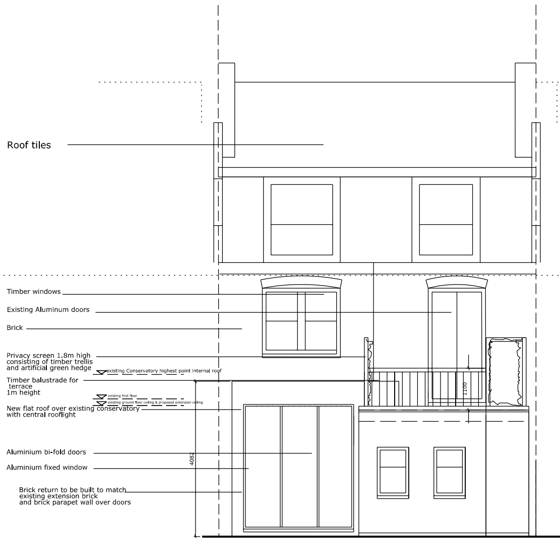
Rear Elevation
