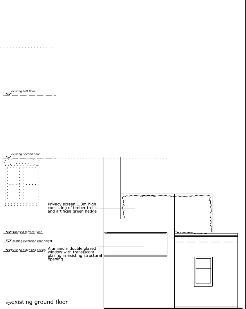
Side Elevation
