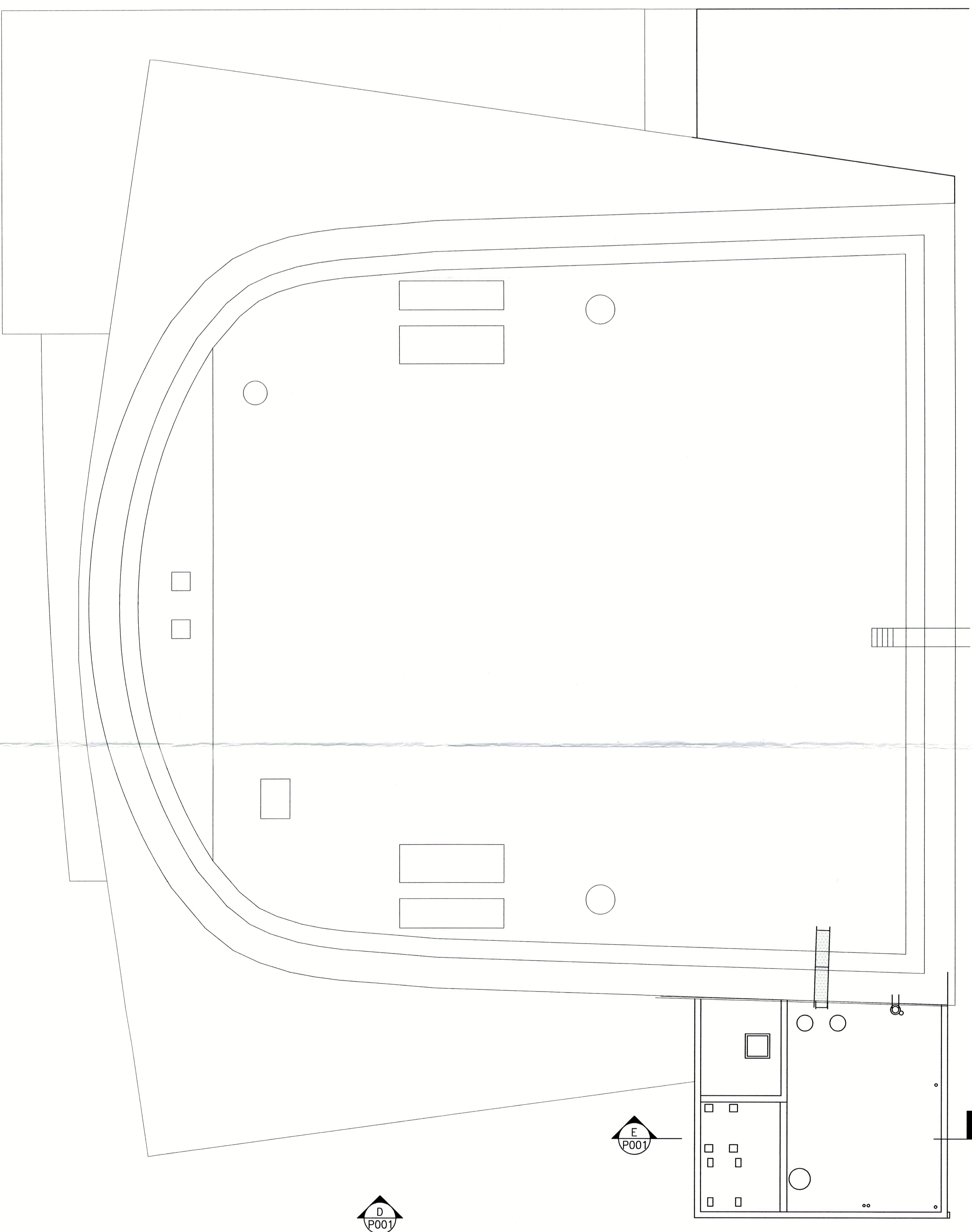
B EXISTING PLAN P001 1:100
