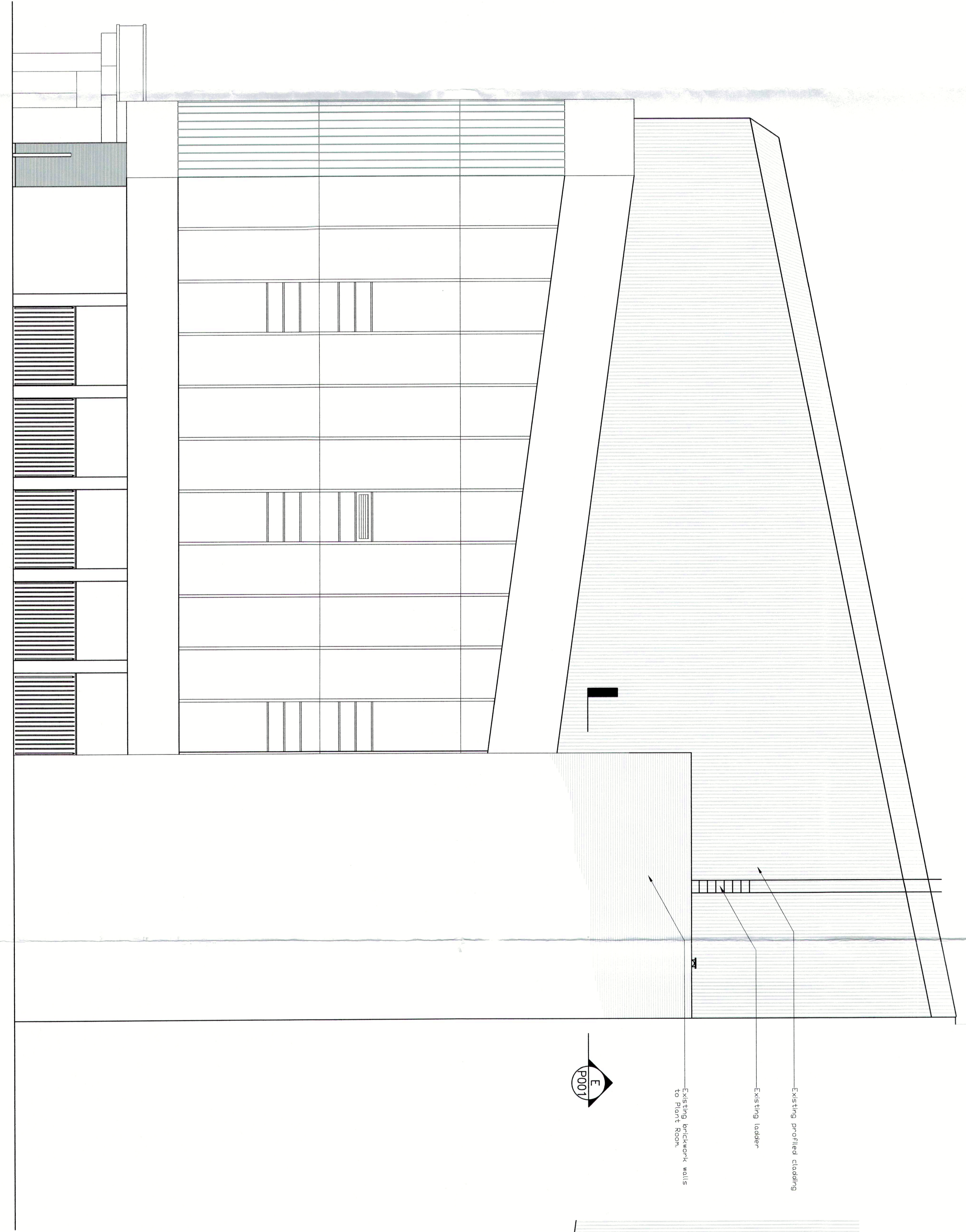
D EAST ELEVATION P001 1:100
