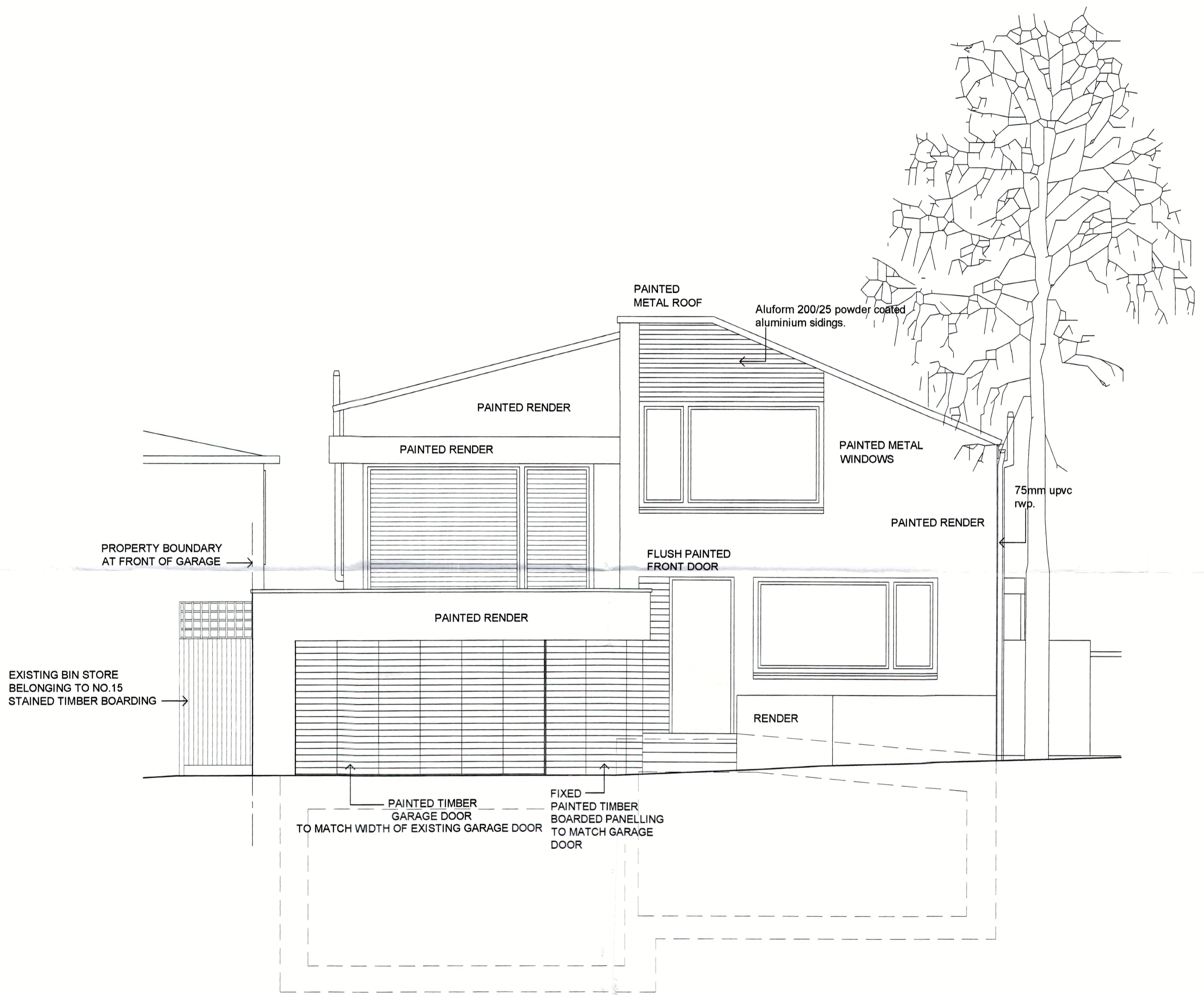
PROPOSED FRONT ELEVATION
