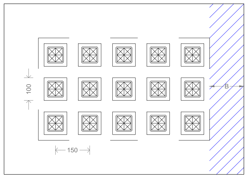
100 x 100 square-lens: 150-mm centres: 100-mm thick
