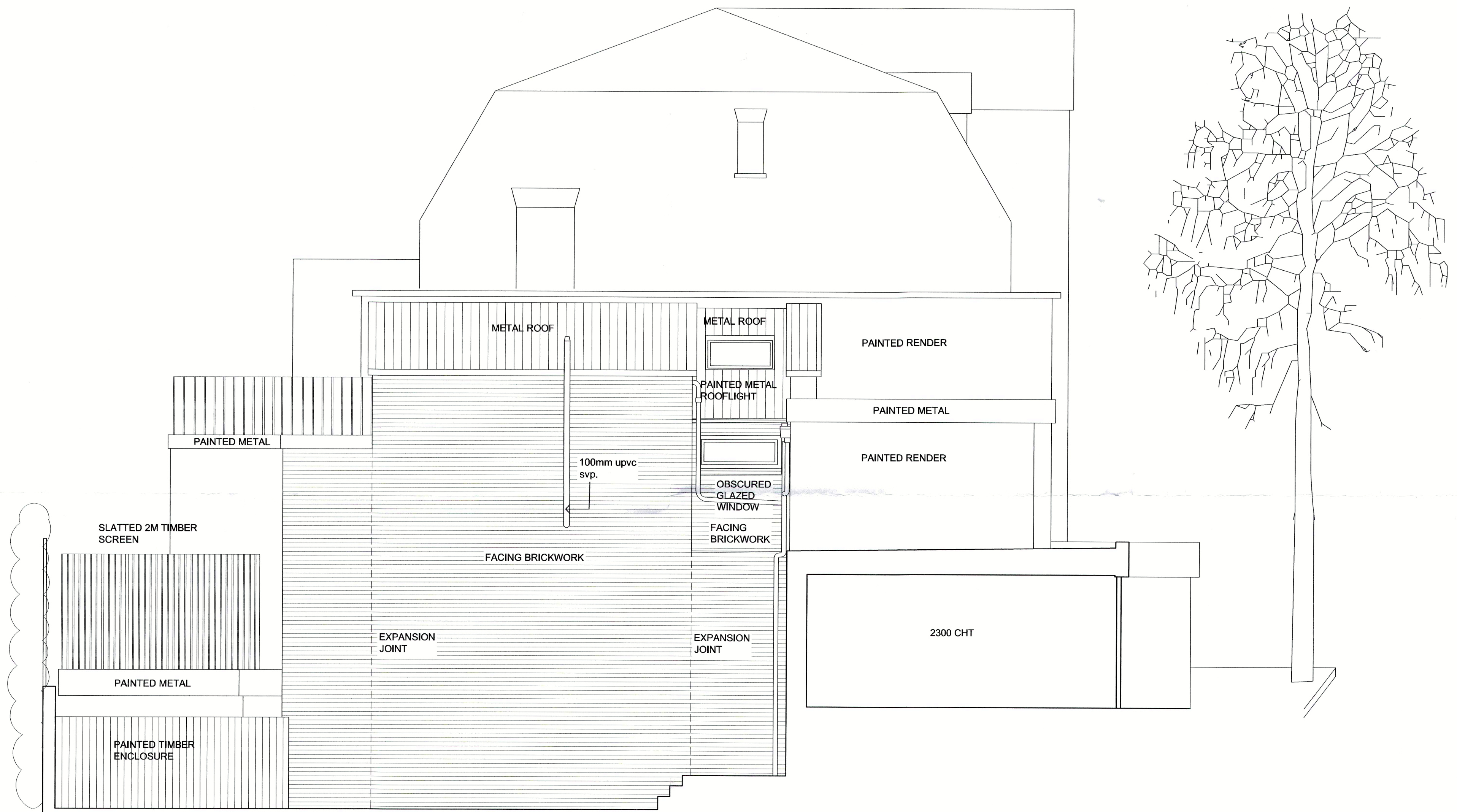
PROPOSED LEFT SIDE ELEVATION
