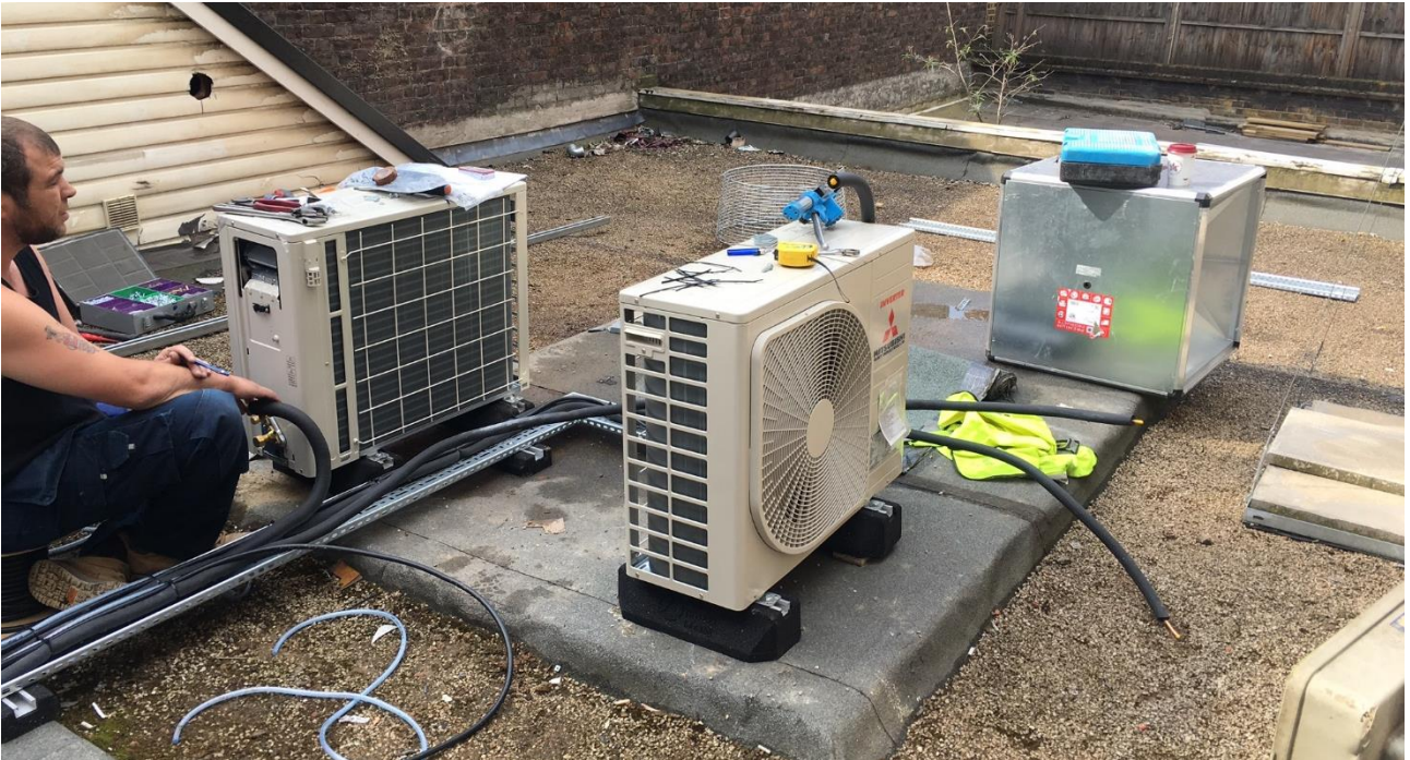
Figure 4; Image of air conditioning condensers on flat roof.
