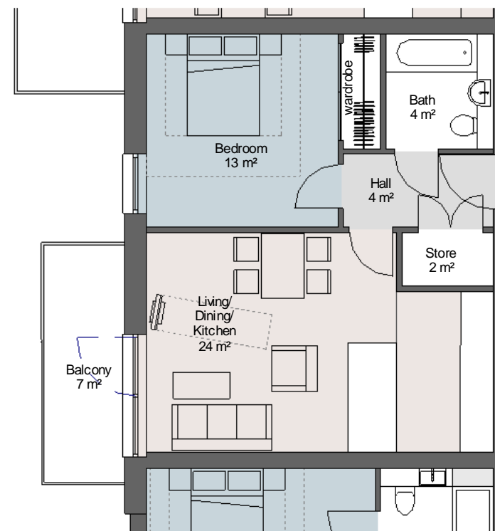
3 Private - Type PP - 1B2P 1 : 100 GIA - 50m²
