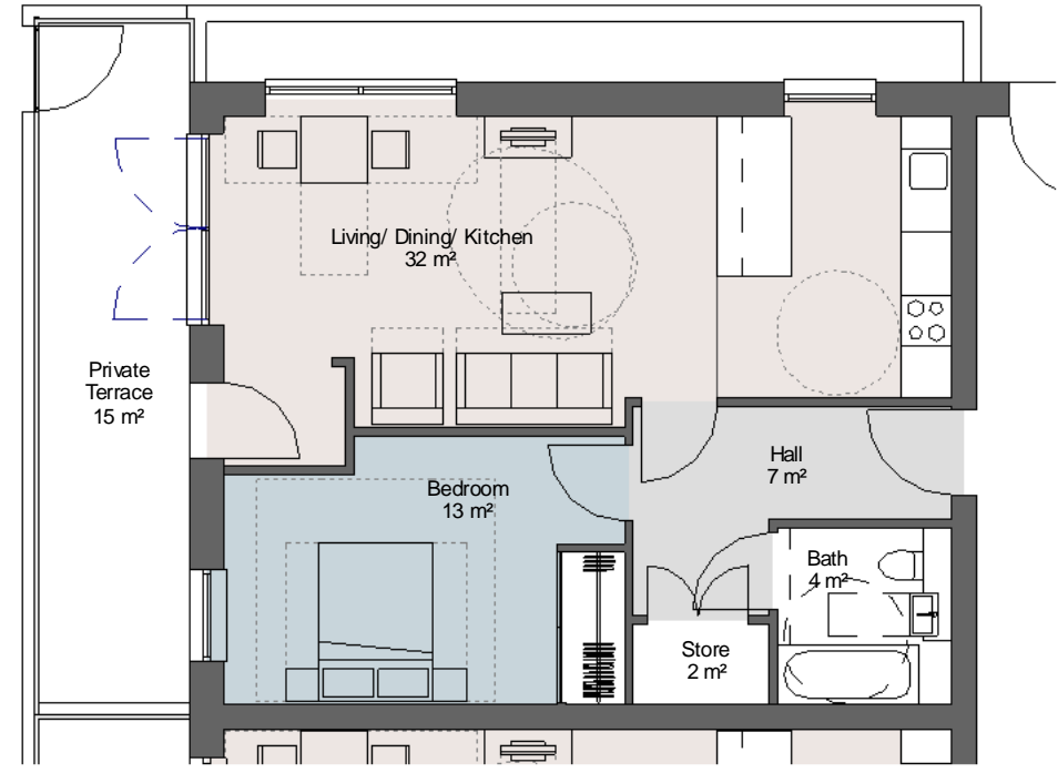
2 Shared Ownership - Type SB North - 1B2P WC 1 : 100 GIA - 61m 2
