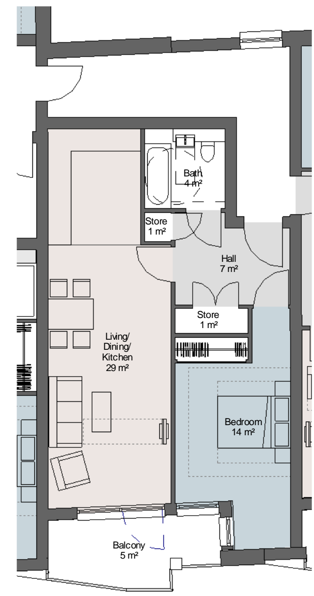
2 Private - Type PI - 1B2P 1 : 100 GIA - 60m 2
