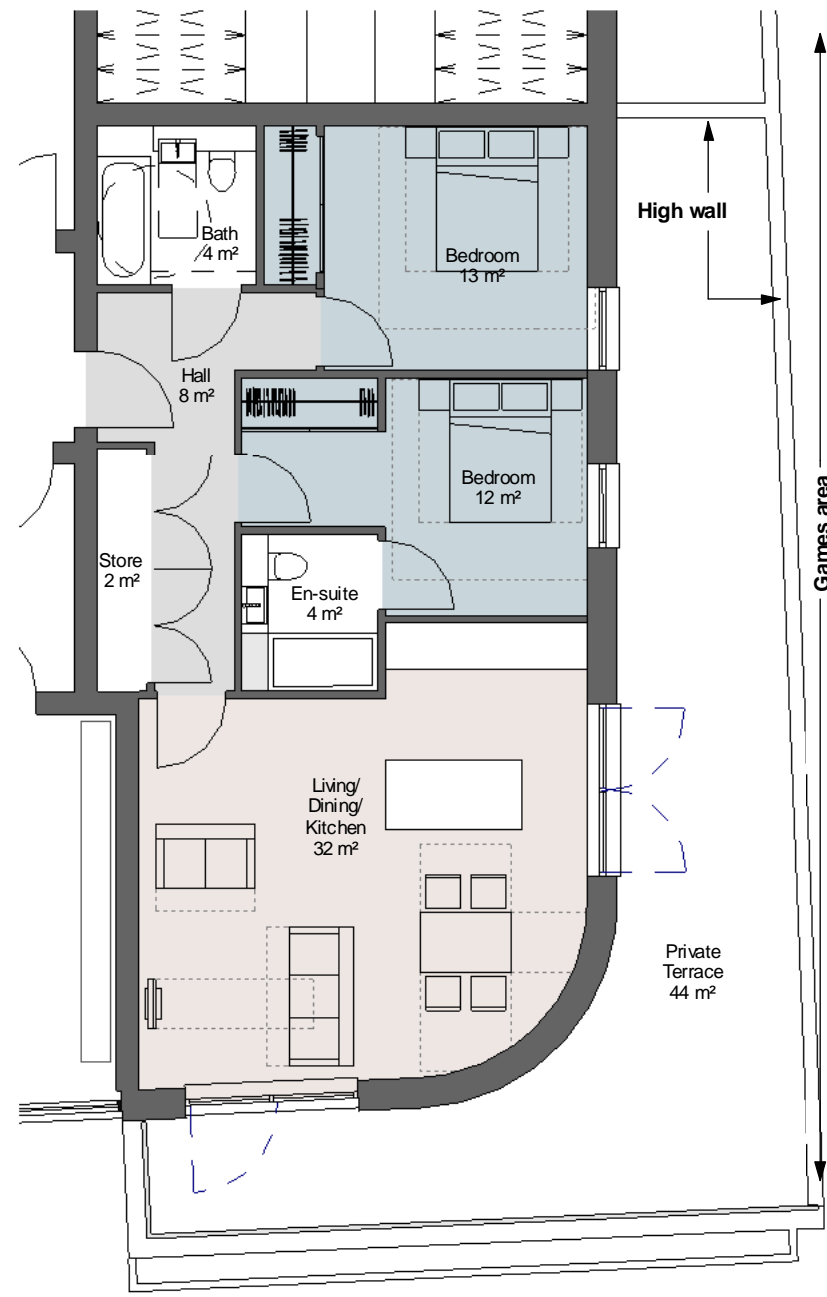
1 Private - Type PB - 2B4P 1 : 100 GIA - 79m 2
