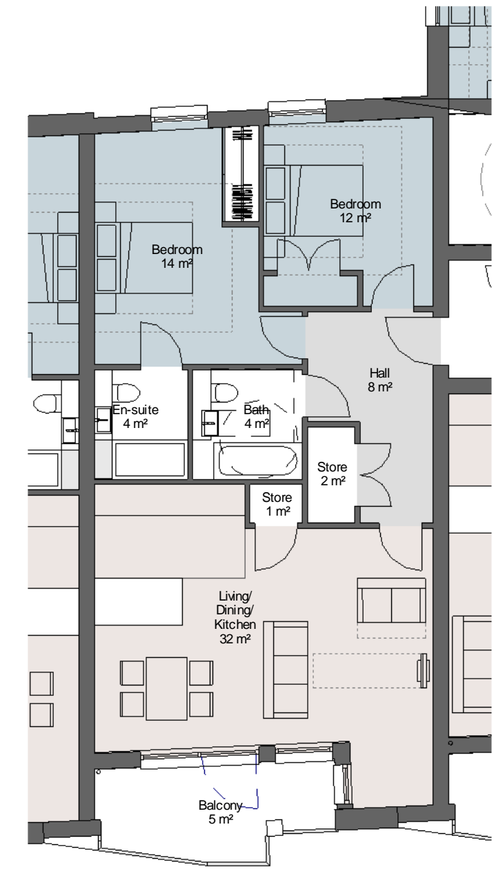
3 Private - Type PJ - 2B4P 1 : 100 GIA - 79m 2
