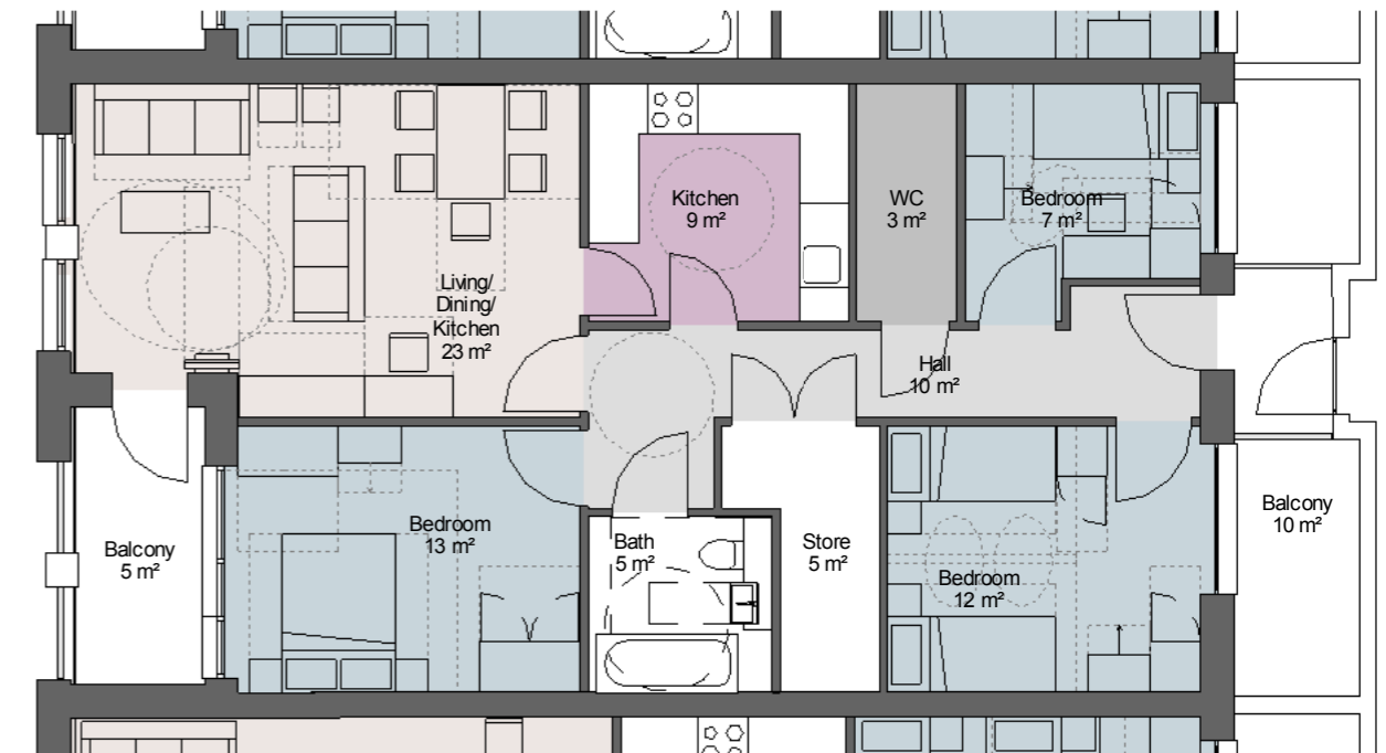
3 Affordable - Type AE2 - 3B5P 1 : 100 GIA - 91m²
