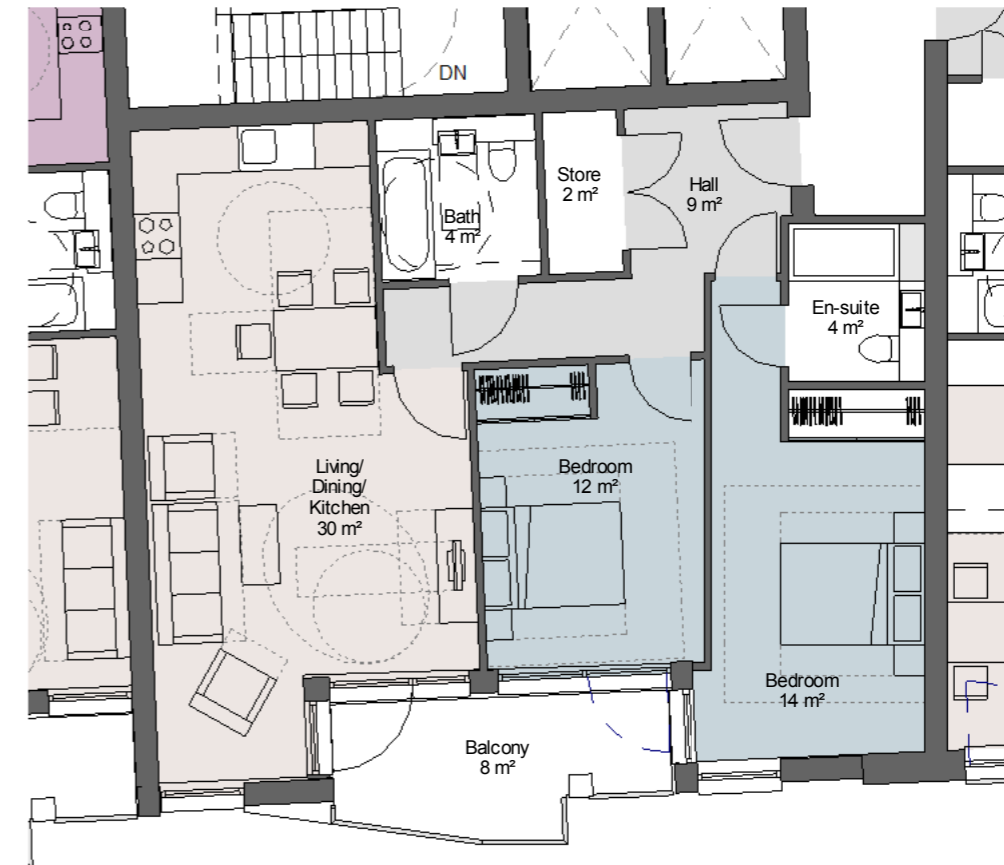
2 Shared Ownership - Type SK - 2B4P 1 : 100 GIA - 79m²
