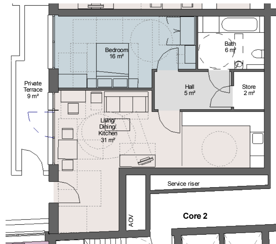
2 Affordable - Type AA - 1B2P - WC 1 : 100 GIA - 65m²
