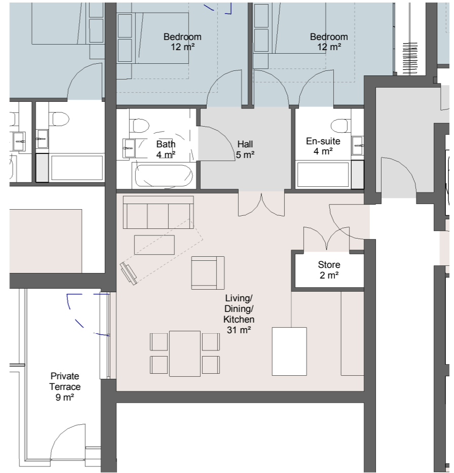
3 Private - Type PD - 2B4P 1 : 100 GIA - 74m²
