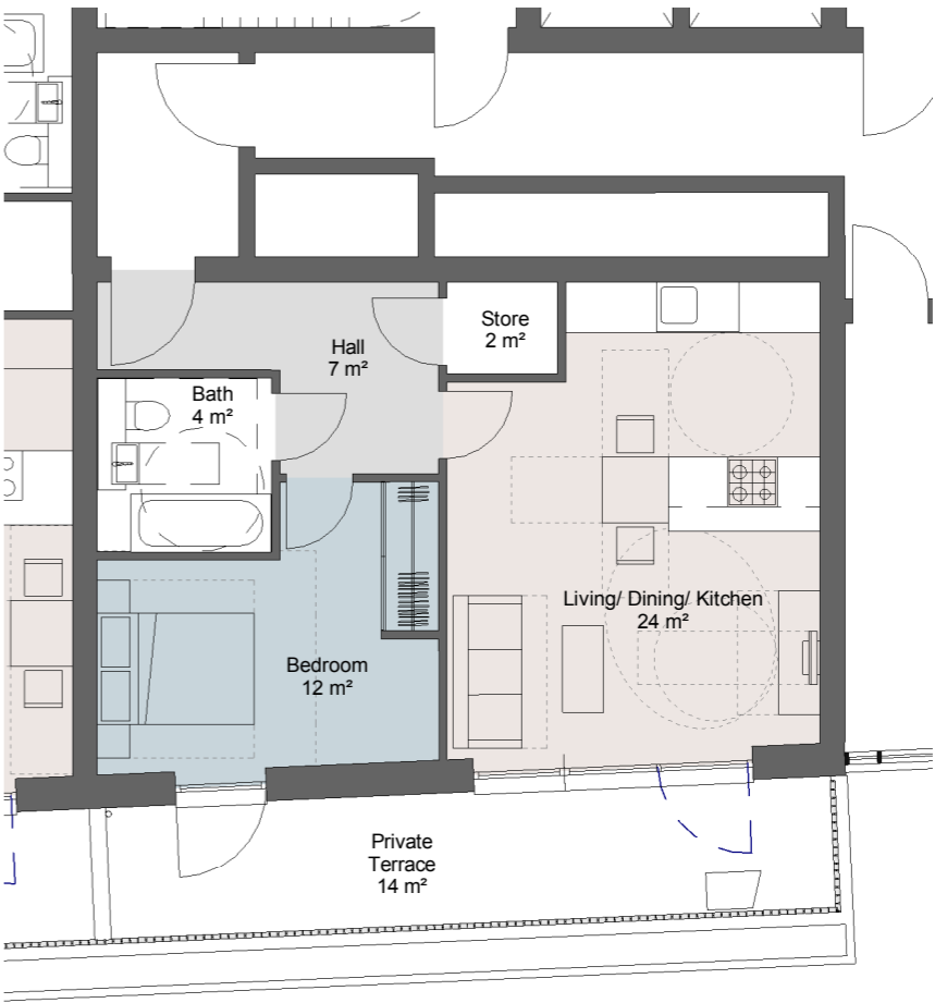
2 Shared Ownership - Type SD - 1B2P 1 : 100 GIA - 51m²
