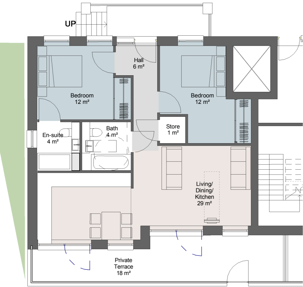
1 Private - Type PC - 2B4P 1 : 100 GIA - 71m²
