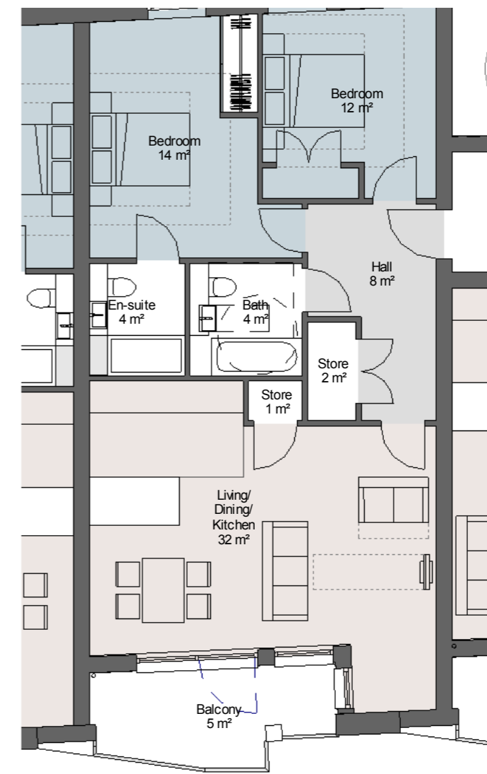
3 Private - Type PJ - 2B4P 1 : 100 GIA - 79m²
