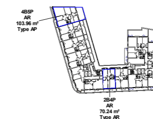
FIFTH FLOOR KEY PLAN
