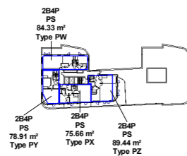
FIFTH FLOOR KEY PLAN
