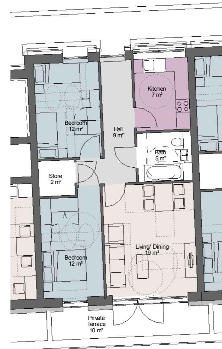
2 Affordable - Type AR - 2B4P 1 : 100
