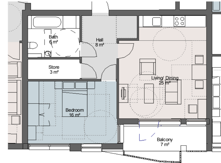
2 Affordable - Type AB - 1B2P - WC 1 : 100 GIA - 59m²
