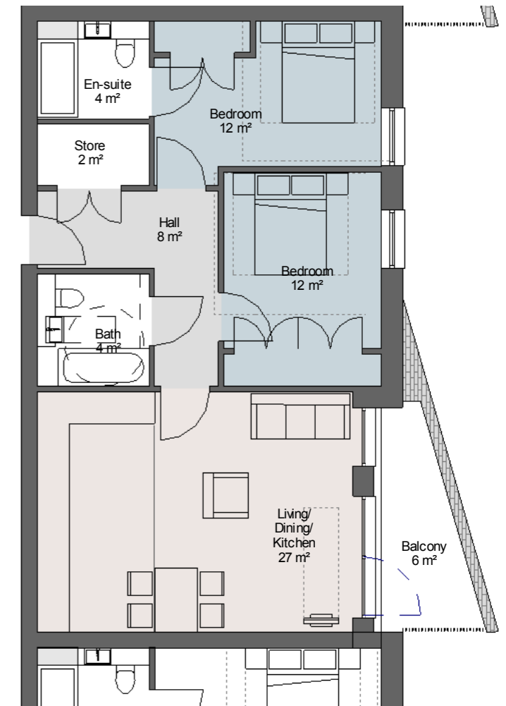
3 Private - Type PL - 2B4P 1 : 100 GIA - 72m²
