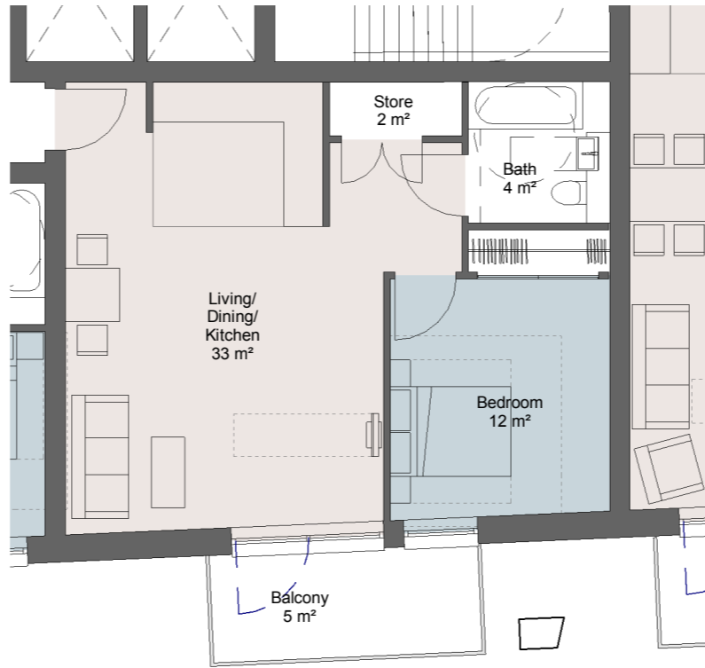
2 Private - Type PH - 1B2P 1 : 100 GIA - 51m²
