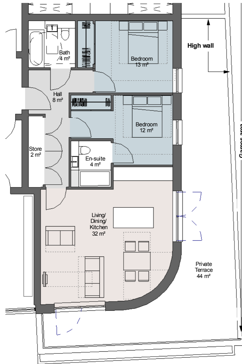
1 Private - Type PB - 2B4P 1 : 100 GIA - 79m²
