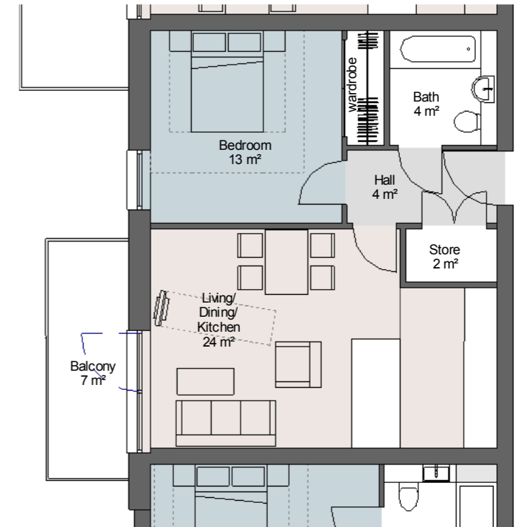
3 Private - Type PP - 1B2P 1 : 100 GIA - 50m²
