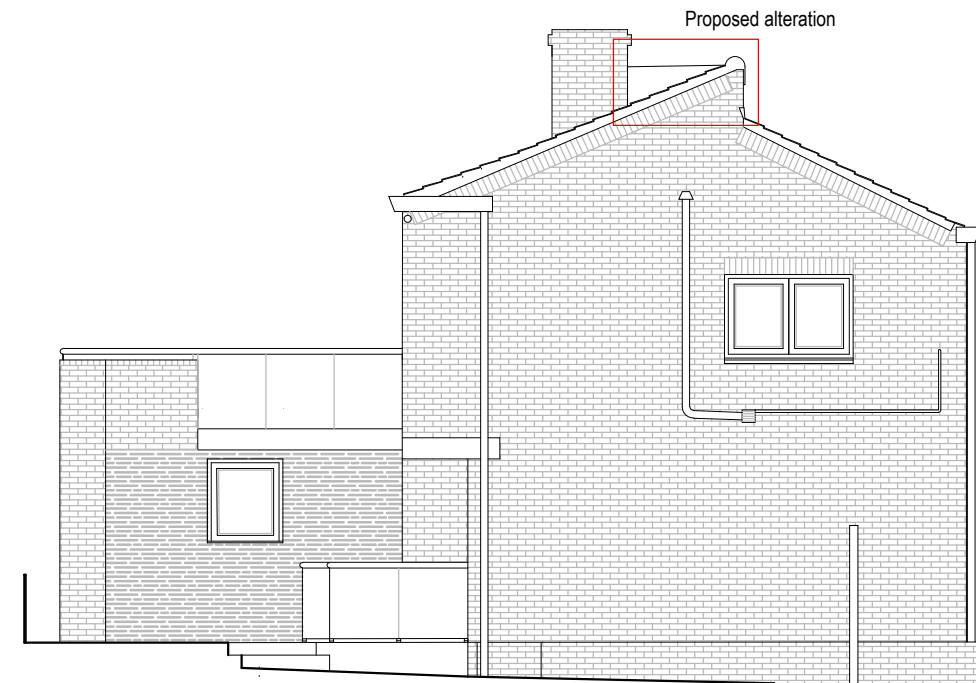
NORTH-WEST ELEVATION
