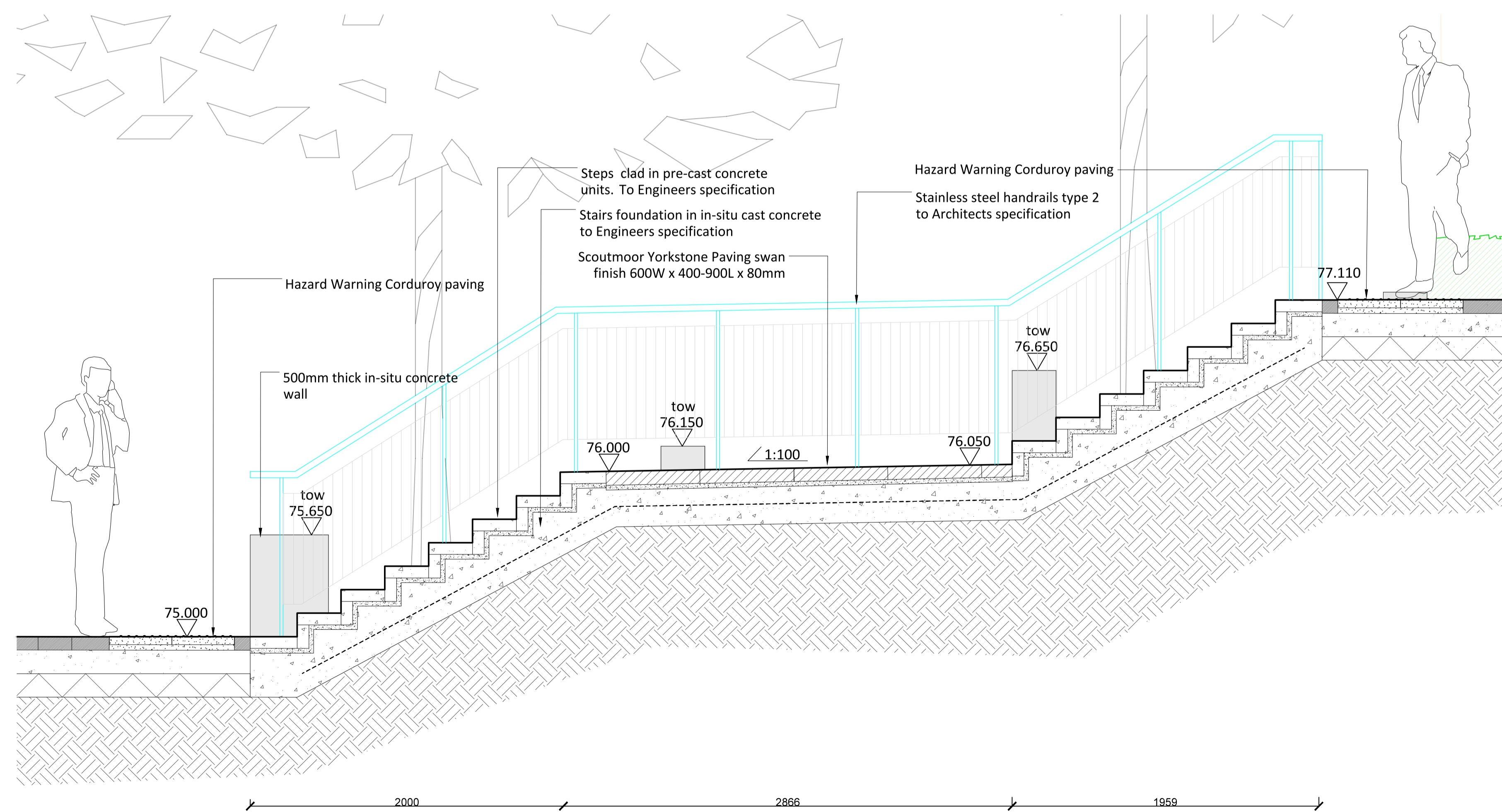
F Scale 1:20
