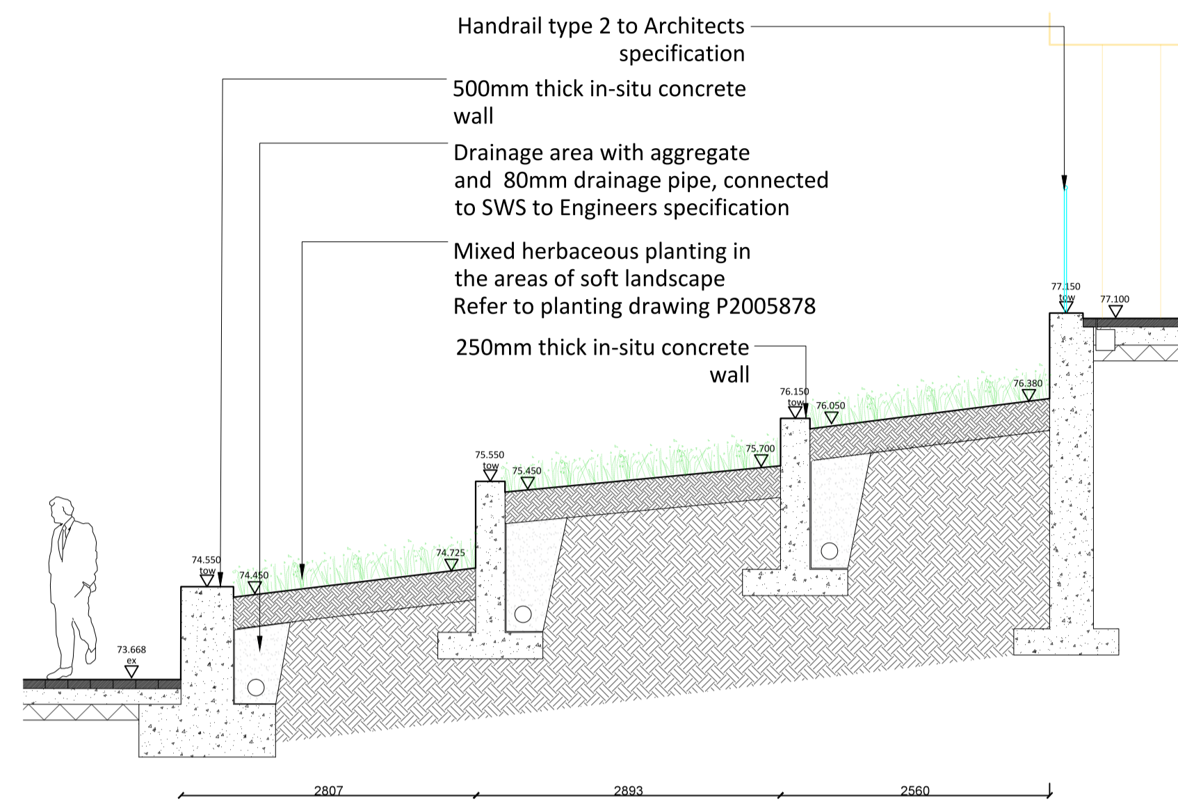
D Scale 1:20
