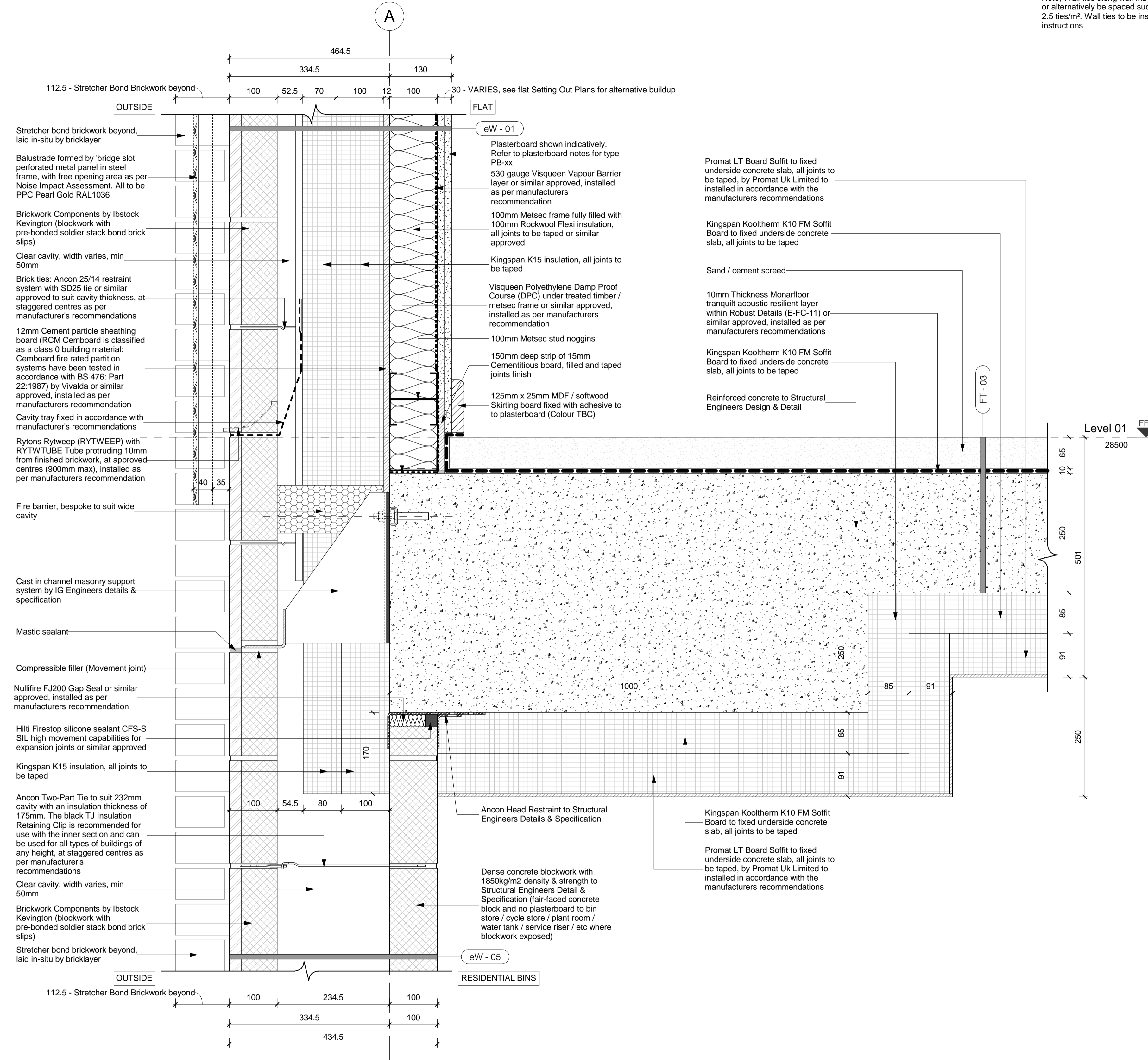
Section of External Wall with Cast in channel masonry support system (Soldier-Course Stack Bond), Slab Edge Detail & Separating Floor between Residential Bins to Flat
