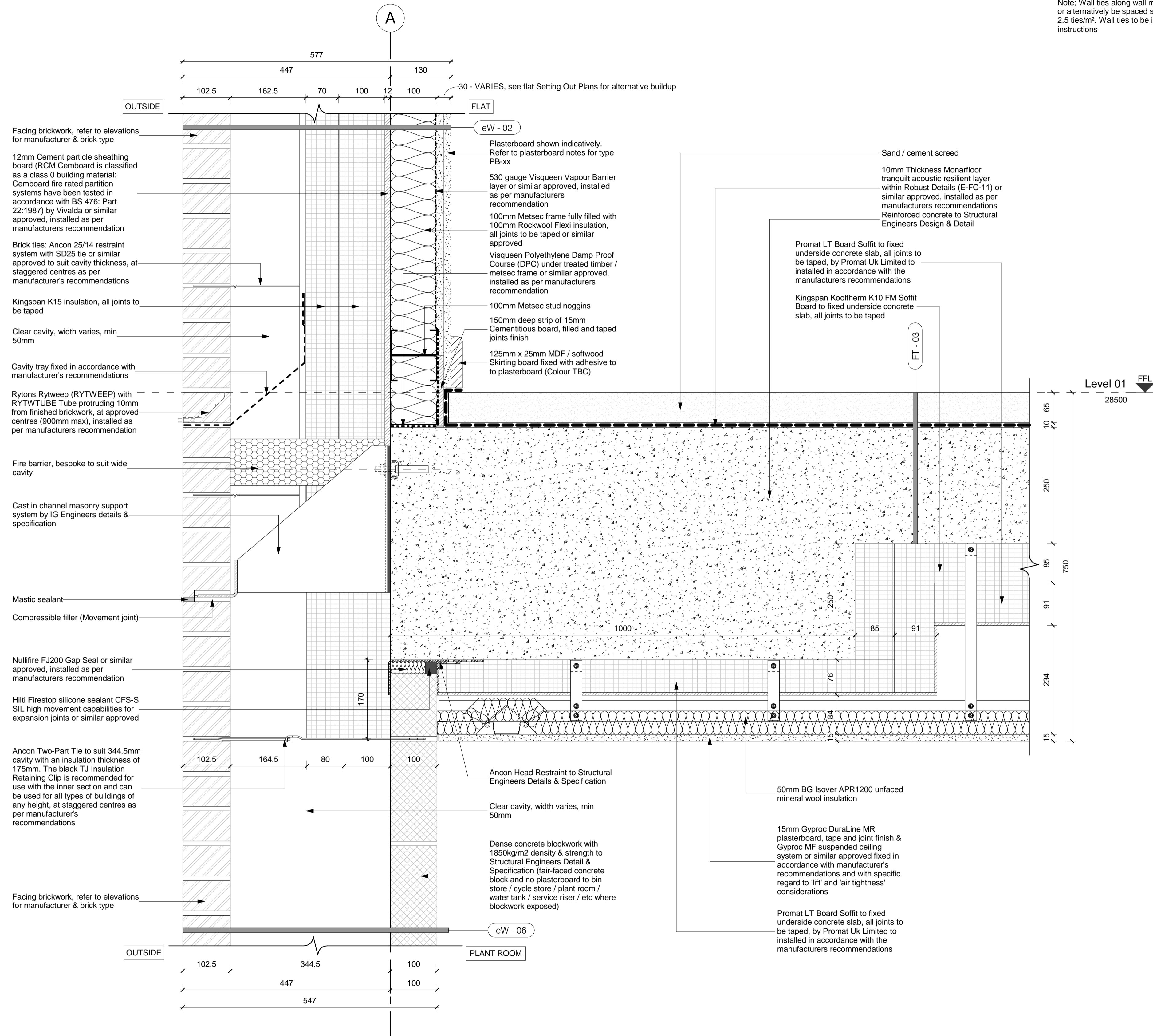
Section of External Wall with Cast in channel masonry support system (Stretcher Bond), Slab Edge Detail & Separating Floor between Plant Room to Flat
