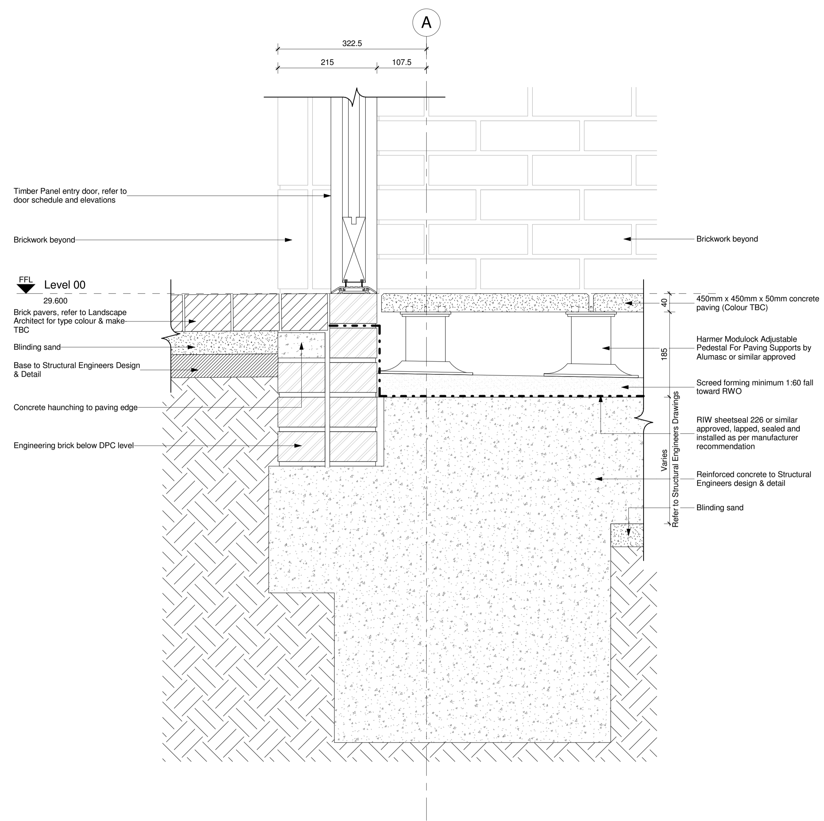
1 Ground Floor Detail - Communal Entry Door 1:5
