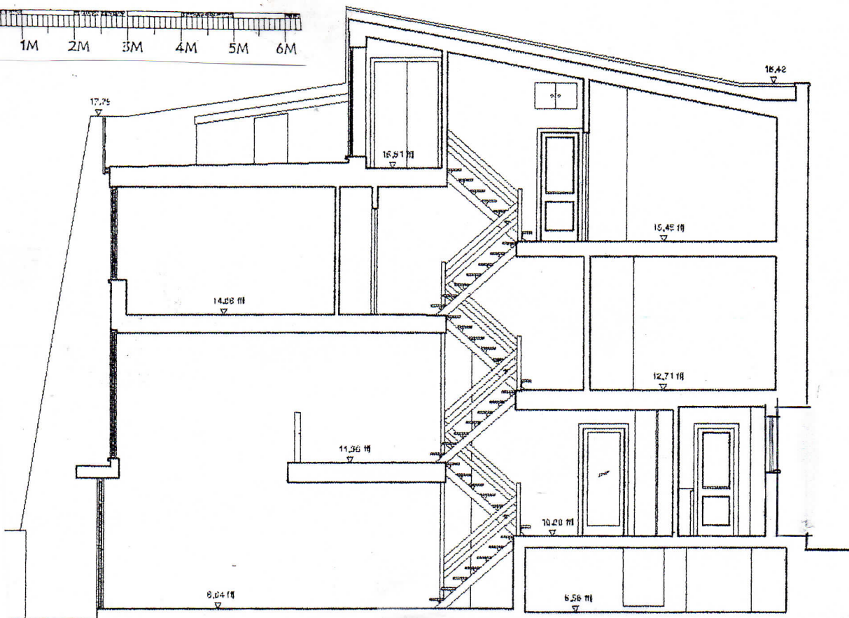
Existing Section
