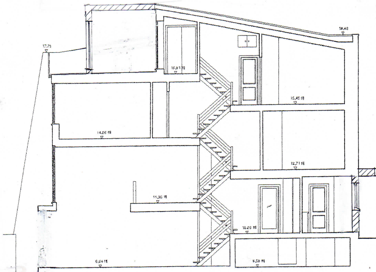
Proposed Section
