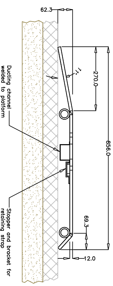
VIEW B-B SCALE 1:10
