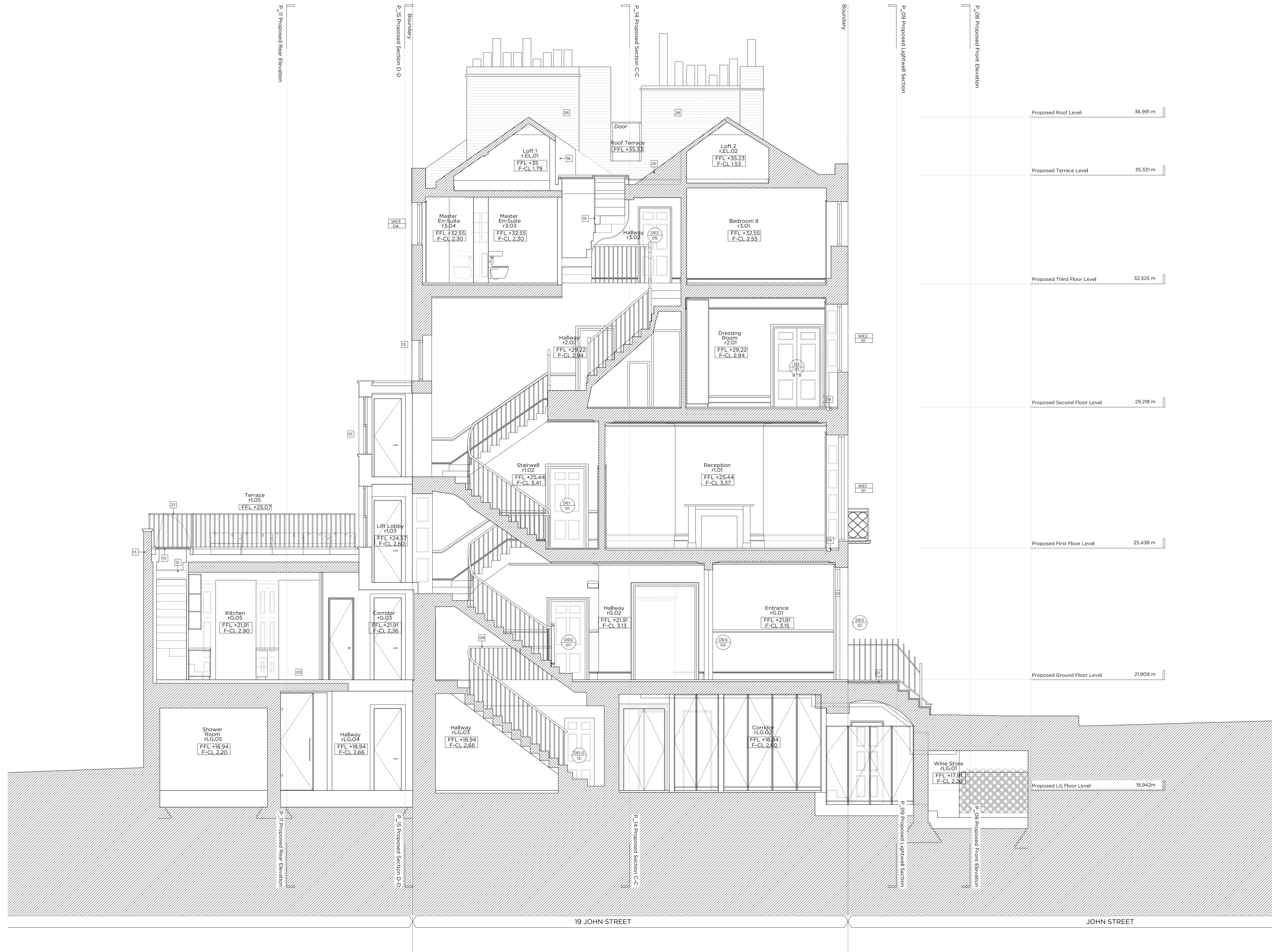
Proposed Section B-B
