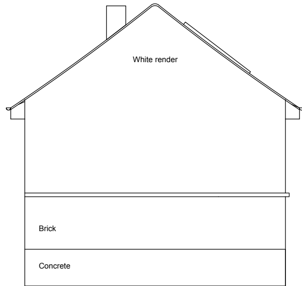
1 West Elevation
